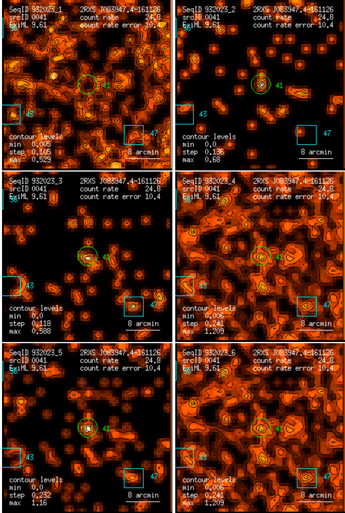
Figure 41: RASS 932023: detection 0041: band rate images, Gaussian filter: (1) PSPC channels 11 – 41, (2) 52 – 90, (3) 91 – 201, (4) 11 – 235, (5) 52 – 201, (6) 11 – 201. Broad band rates in counts/ks. Band rate contour levels in counts/ks/arcmin 2 .
