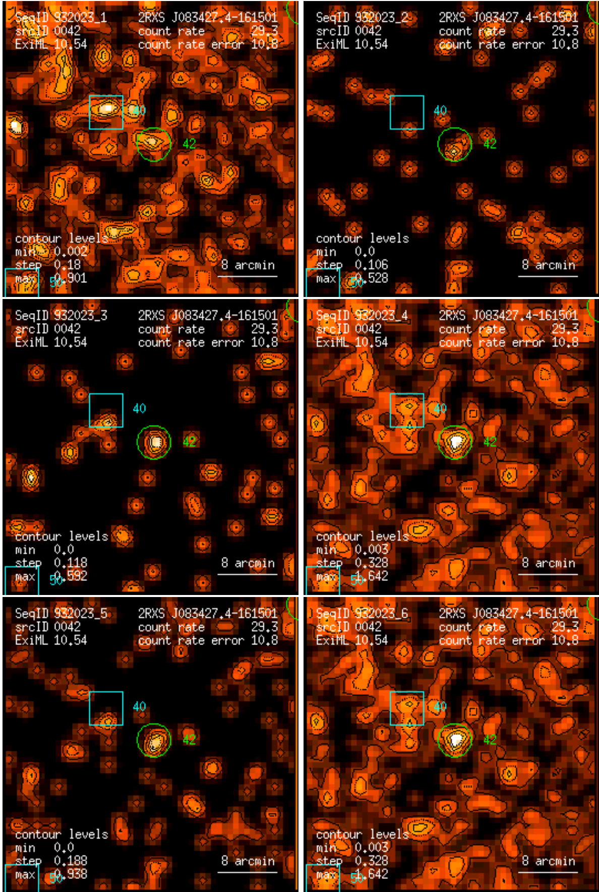
Figure 42: RASS 932023: detection 0042: band rate images, Gaussian filter: (1) PSPC channels 11 – 41, (2) 52 – 90, (3) 91 – 201, (4) 11 – 235, (5) 52 – 201, (6) 11 – 201. Broad band rates in counts/ks. Band rate contour levels in counts/ks/arcmin 2 .
