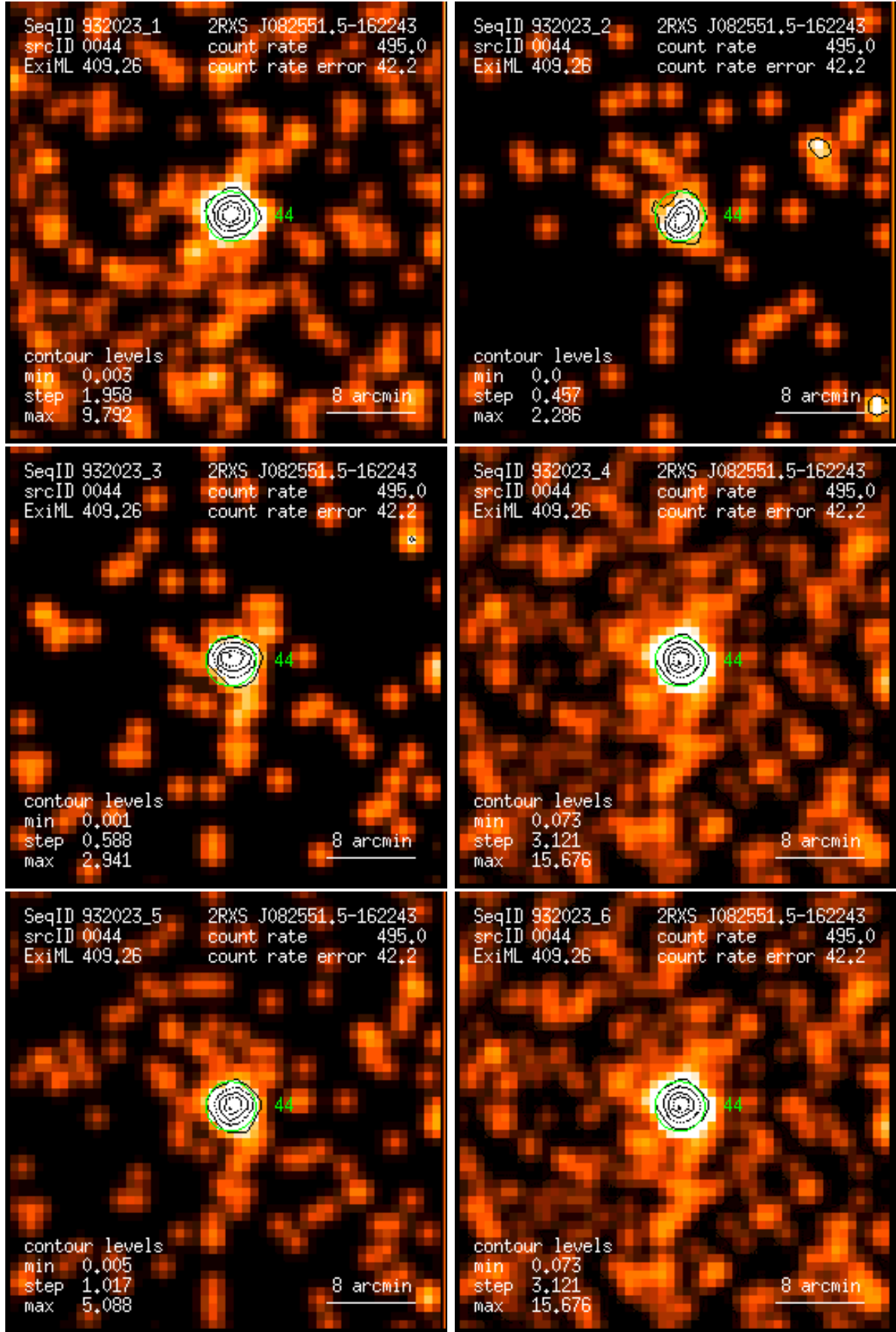
Figure 44: RASS 932023: detection 0044: band rate images, Gaussian filter: (1) PSPC channels 11 – 41, (2) 52 – 90, (3) 91 – 201, (4) 11 – 235, (5) 52 – 201, (6) 11 – 201. Broad band rates in counts/ks. Band rate contour levels in counts/ks/arcmin 2 .
