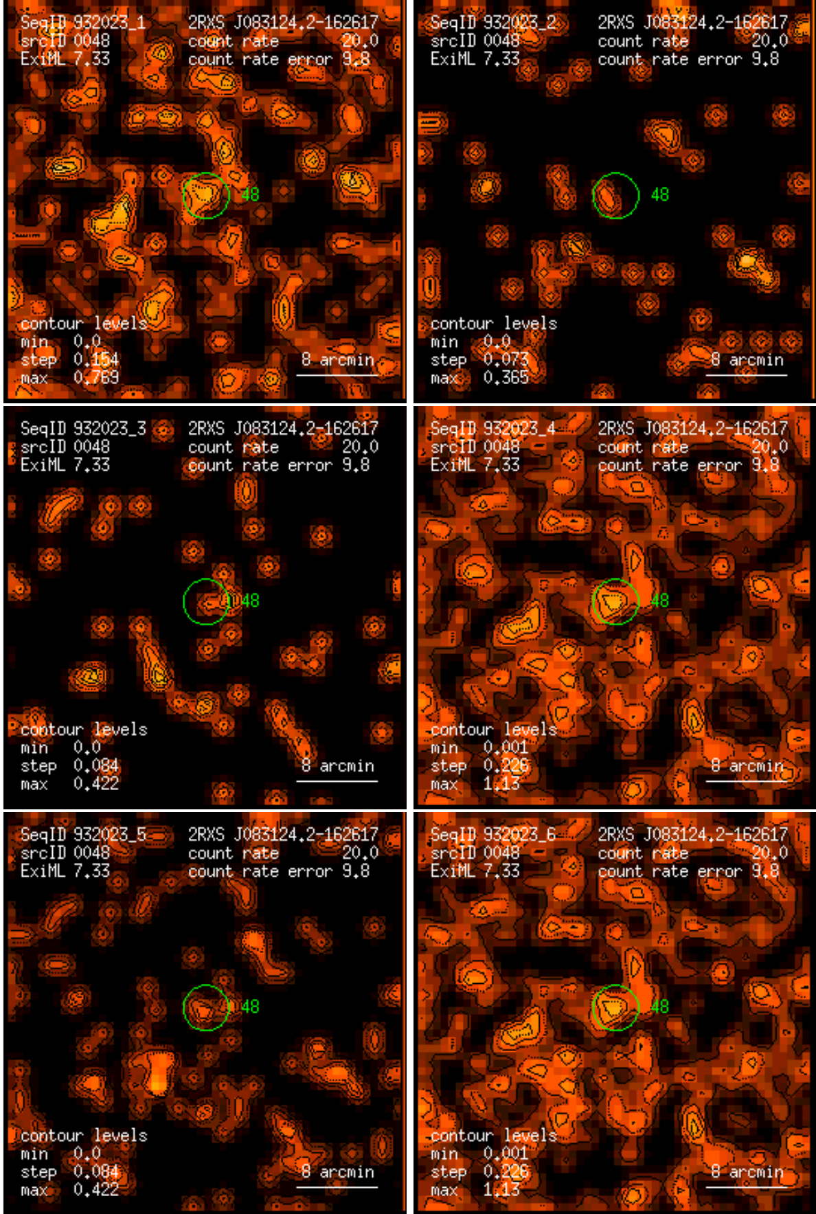
Figure 48: RASS 932023: detection 0048: band rate images, Gaussian filter: (1) PSPC channels 11 – 41, (2) 52 – 90, (3) 91 – 201, (4) 11 – 235, (5) 52 – 201, (6) 11 – 201. Broad band rates in counts/ks. Band rate contour levels in counts/ks/arcmin 2 .
