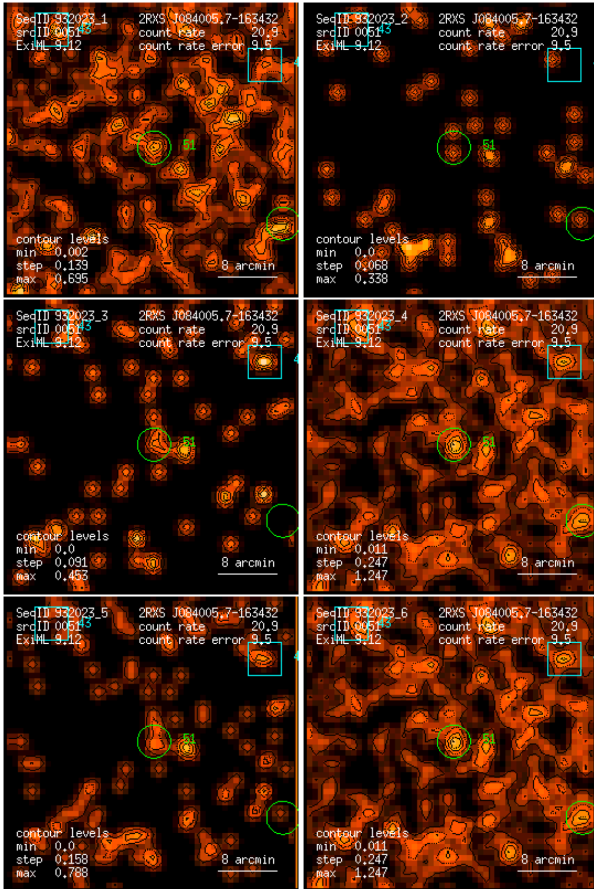
Figure 51: RASS 932023: detection 0051: band rate images, Gaussian filter: (1) PSPC channels 11 – 41, (2) 52 – 90, (3) 91 – 201, (4) 11 – 235, (5) 52 – 201, (6) 11 – 201. Broad band rates in counts/ks. Band rate contour levels in counts/ks/arcmin 2 .
