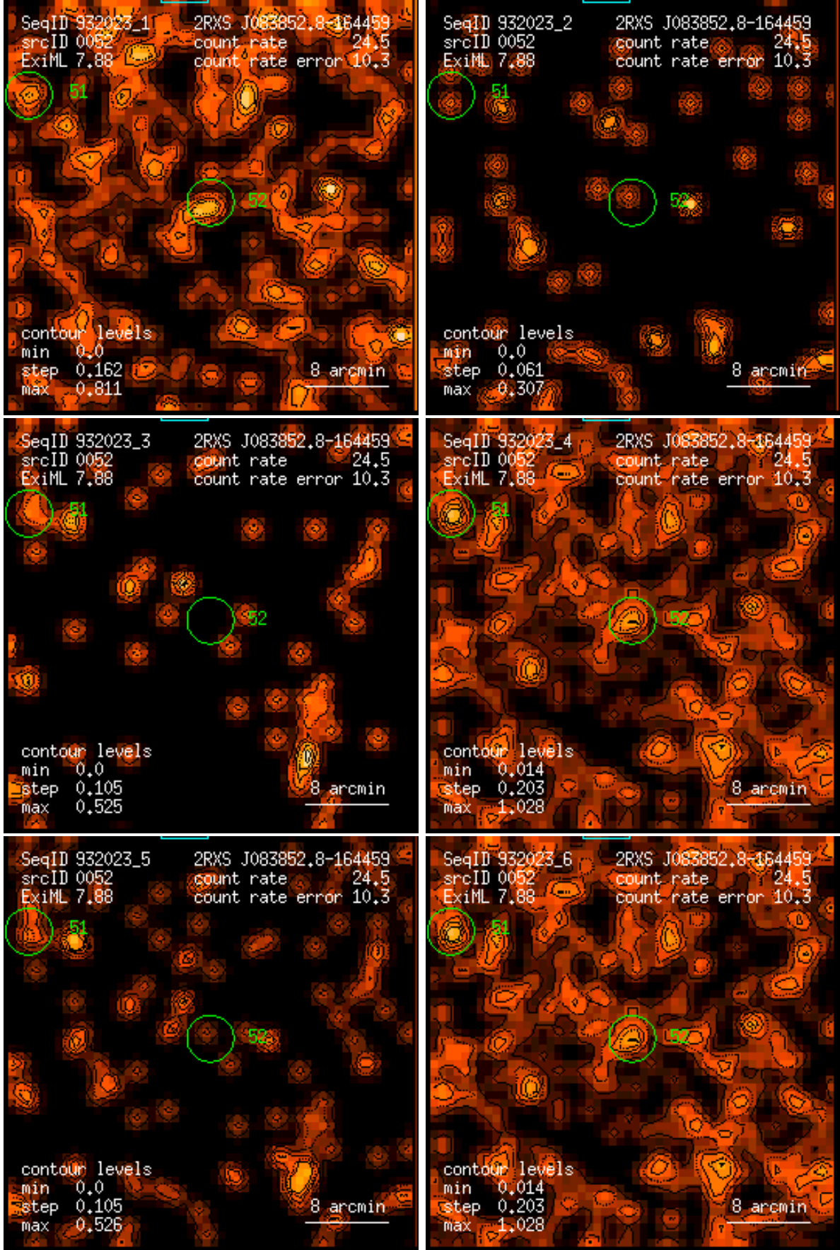
Figure 52: RASS 932023: detection 0052: band rate images, Gaussian filter: (1) PSPC channels 11 – 41, (2) 52 – 90, (3) 91 – 201, (4) 11 – 235, (5) 52 – 201, (6) 11 – 201. Broad band rates in counts/ks. Band rate contour levels in counts/ks/arcmin 2 .
