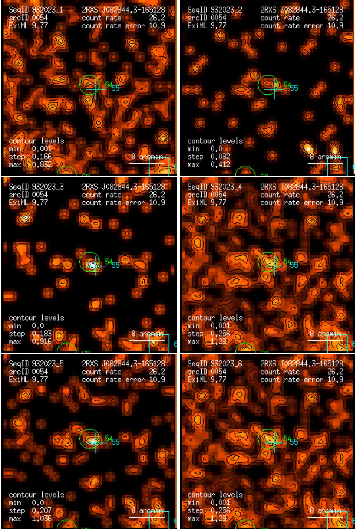
Figure 54: RASS 932023: detection 0054: band rate images, Gaussian filter: (1) PSPC channels 11 – 41, (2) 52 – 90, (3) 91 – 201, (4) 11 – 235, (5) 52 – 201, (6) 11 – 201. Broad band rates in counts/ks. Band rate contour levels in counts/ks/arcmin 2 .
