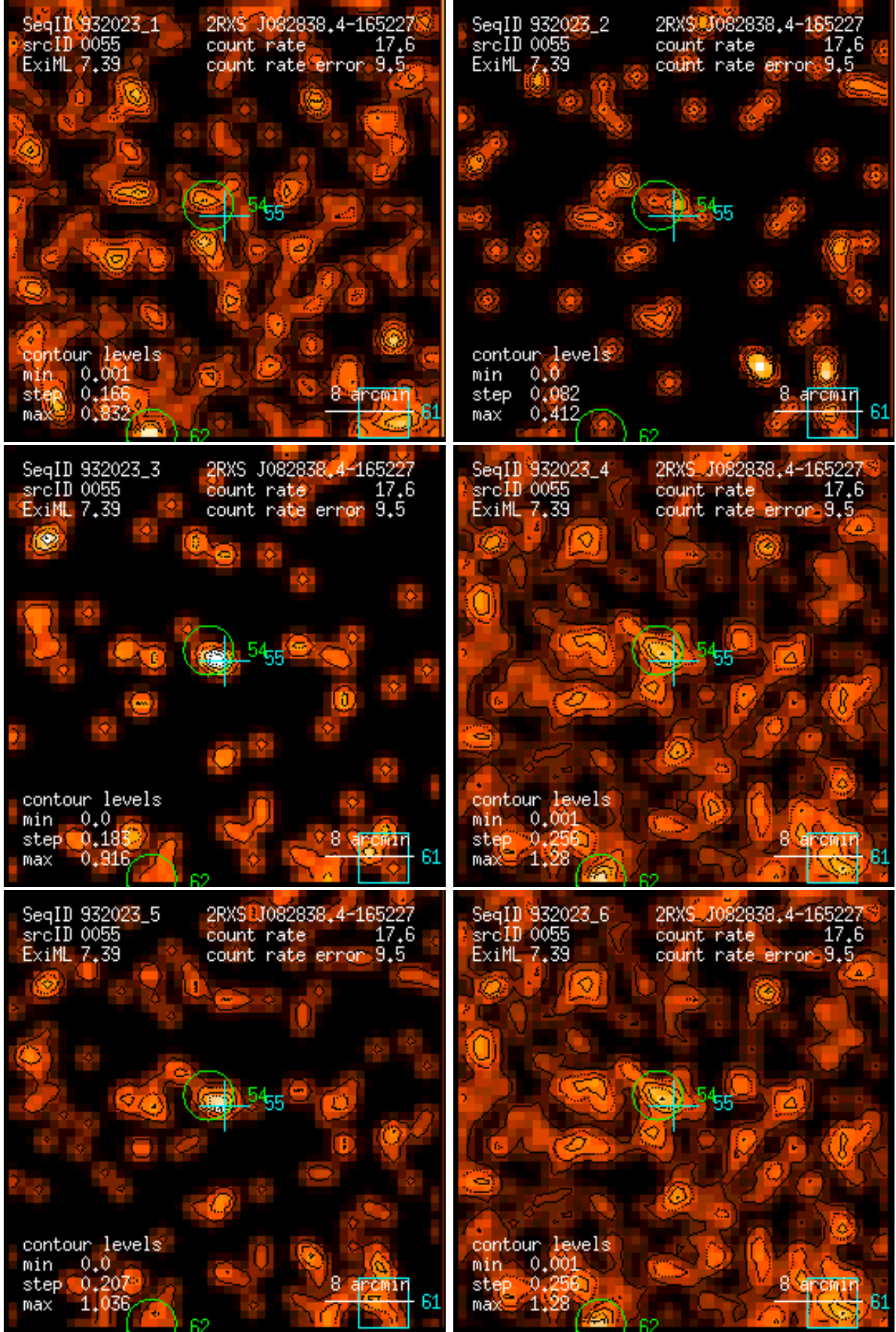
Figure 55: RASS 932023: detection 0055: band rate images, Gaussian filter: (1) PSPC channels 11 – 41, (2) 52 – 90, (3) 91 – 201, (4) 11 – 235, (5) 52 – 201, (6) 11 – 201. Broad band rates in counts/ks. Band rate contour levels in counts/ks/arcmin 2 .
