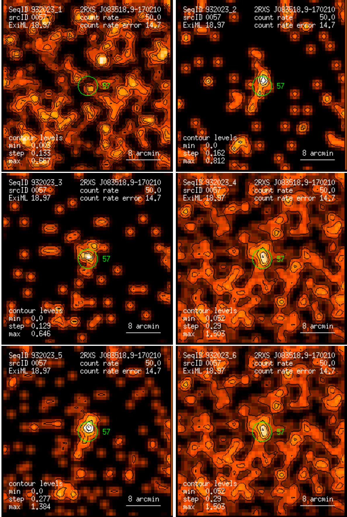
Figure 57: RASS 932023: detection 0057: band rate images, Gaussian filter: (1) PSPC channels 11 – 41, (2) 52 – 90, (3) 91 – 201, (4) 11 – 235, (5) 52 – 201, (6) 11 – 201. Broad band rates in counts/ks. Band rate contour levels in counts/ks/arcmin 2 .
