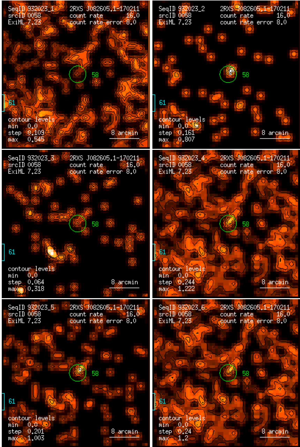
Figure 58: RASS 932023: detection 0058: band rate images, Gaussian filter: (1) PSPC channels 11 – 41, (2) 52 – 90, (3) 91 – 201, (4) 11 – 235, (5) 52 – 201, (6) 11 – 201. Broad band rates in counts/ks. Band rate contour levels in counts/ks/arcmin 2 .
