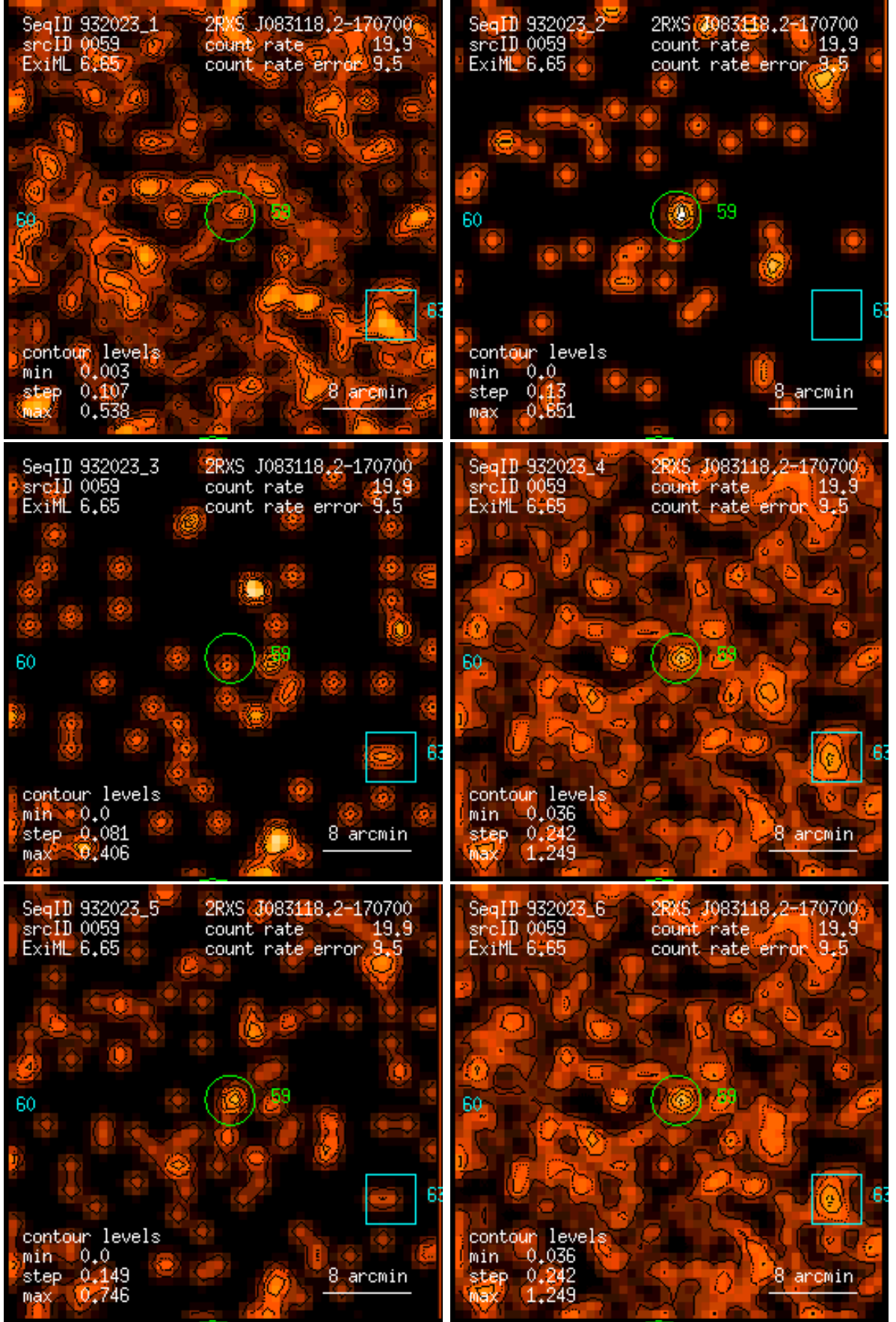
Figure 59: RASS 932023: detection 0059: band rate images, Gaussian filter: (1) PSPC channels 11 – 41, (2) 52 – 90, (3) 91 – 201, (4) 11 – 235, (5) 52 – 201, (6) 11 – 201. Broad band rates in counts/ks. Band rate contour levels in counts/ks/arcmin 2 .
