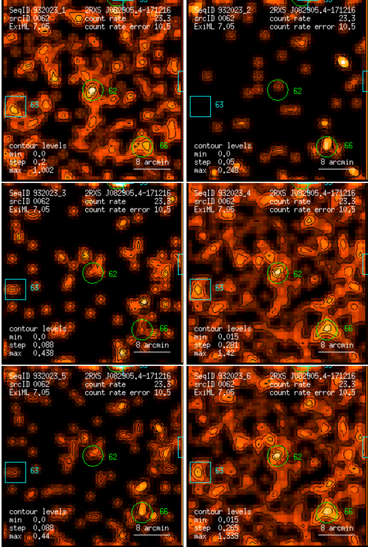
Figure 62: RASS 932023: detection 0062: band rate images, Gaussian filter: (1) PSPC channels 11 – 41, (2) 52 – 90, (3) 91 – 201, (4) 11 – 235, (5) 52 – 201, (6) 11 – 201. Broad band rates in counts/ks. Band rate contour levels in counts/ks/arcmin 2 .
