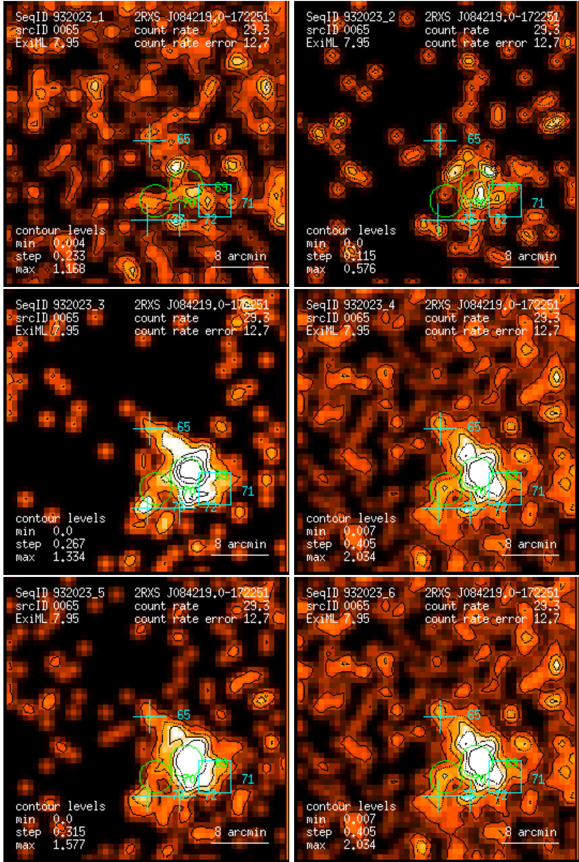
Figure 65: RASS 932023: detection 0065: band rate images, Gaussian filter: (1) PSPC channels 11 – 41, (2) 52 – 90, (3) 91 – 201, (4) 11 – 235, (5) 52 – 201, (6) 11 – 201. Broad band rates in counts/ks. Band rate contour levels in counts/ks/arcmin 2 .
