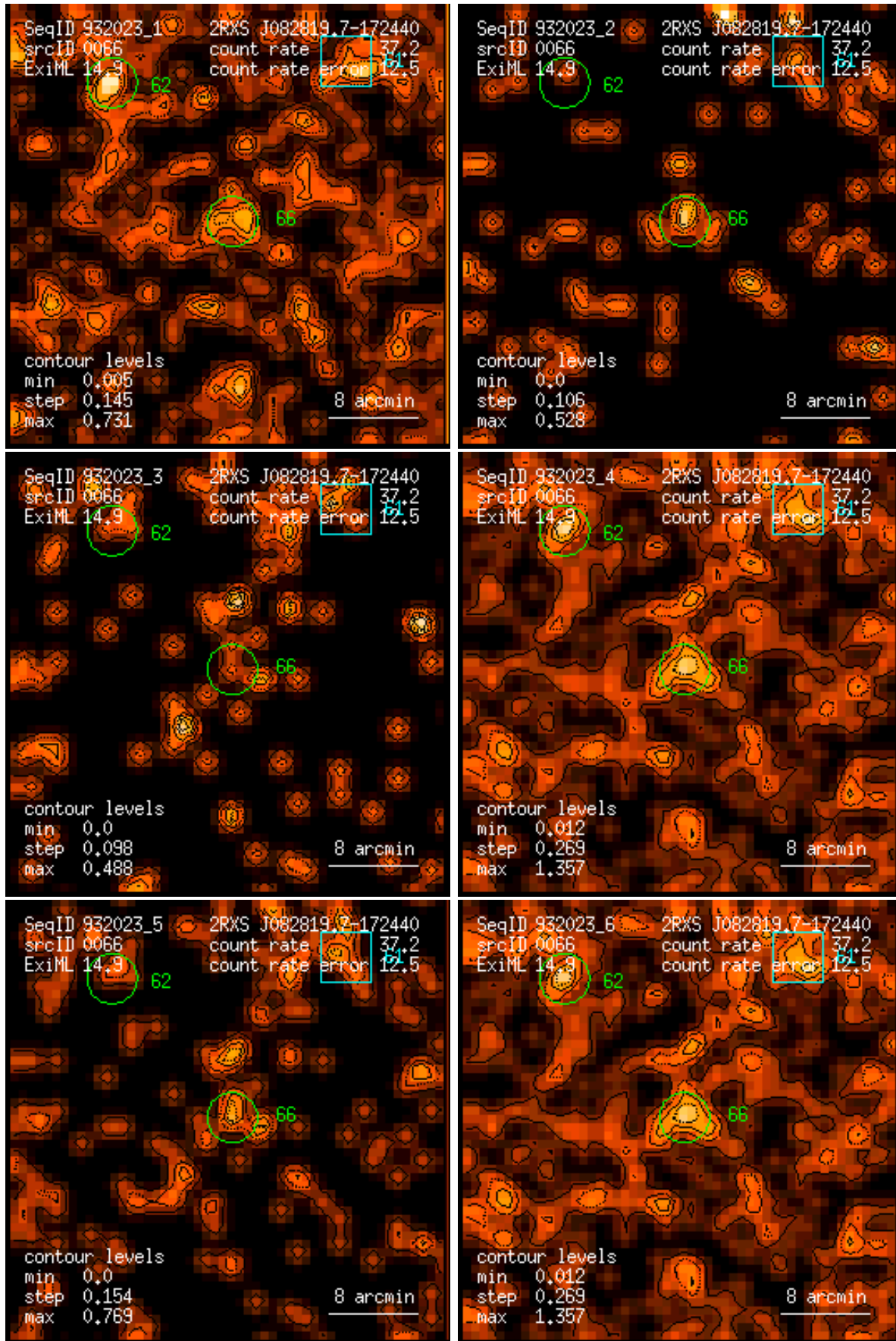
Figure 66: RASS 932023: detection 0066: band rate images, Gaussian filter: (1) PSPC channels 11 – 41, (2) 52 – 90, (3) 91 – 201, (4) 11 – 235, (5) 52 – 201, (6) 11 – 201. Broad band rates in counts/ks. Band rate contour levels in counts/ks/arcmin 2 .
