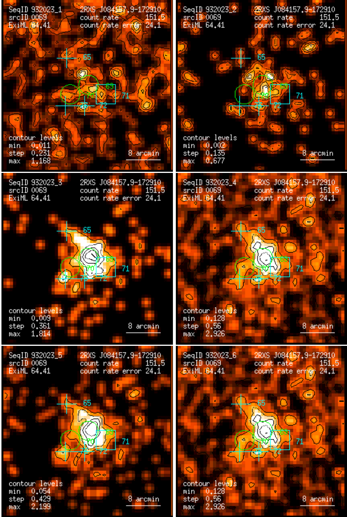
Figure 69: RASS 932023: detection 0069: band rate images, Gaussian filter: (1) PSPC channels 11 – 41, (2) 52 – 90, (3) 91 – 201, (4) 11 – 235, (5) 52 – 201, (6) 11 – 201. Broad band rates in counts/ks. Band rate contour levels in counts/ks/arcmin 2 .
