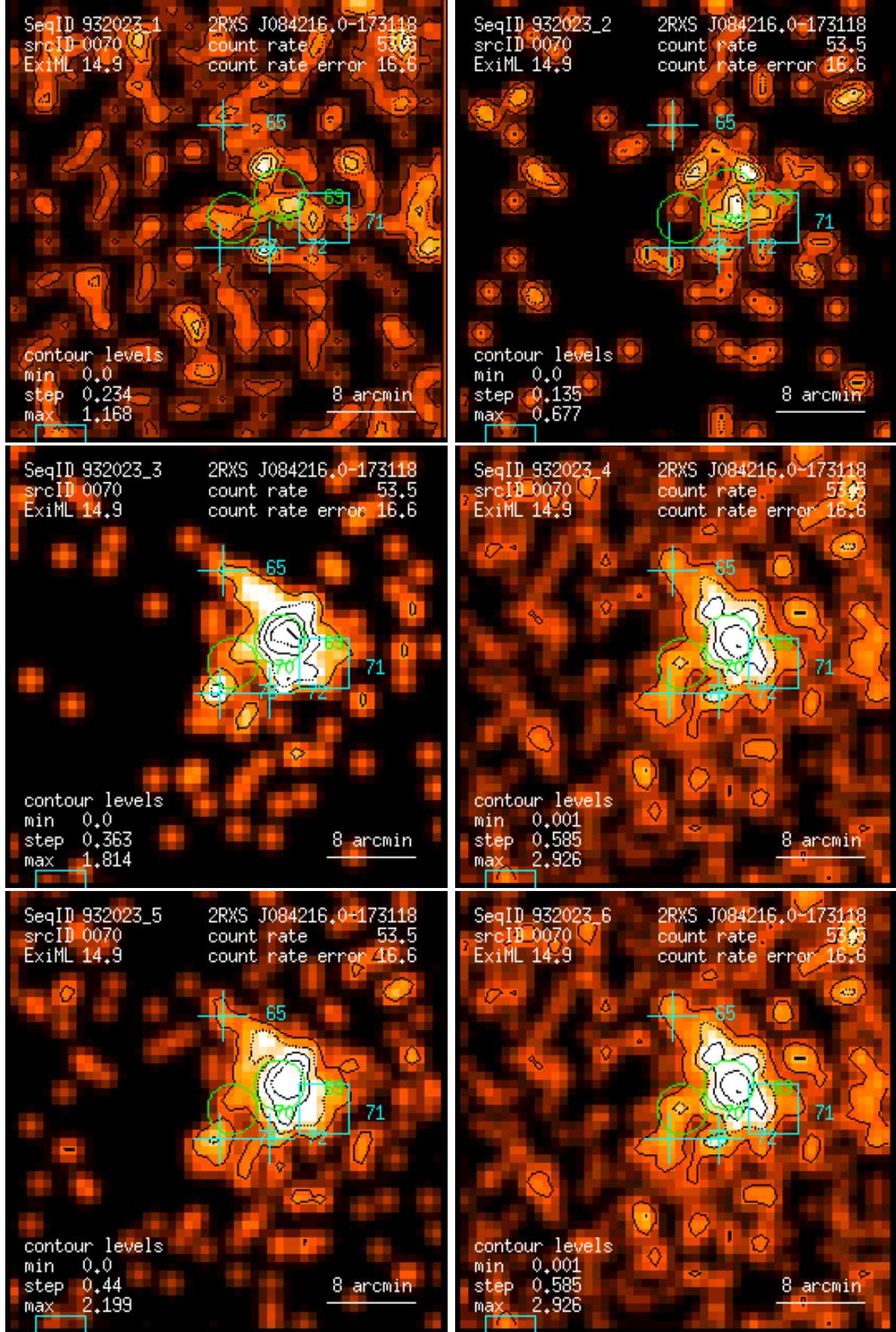
Figure 70: RASS 932023: detection 0070: band rate images, Gaussian filter: (1) PSPC channels 11 – 41, (2) 52 – 90, (3) 91 – 201, (4) 11 – 235, (5) 52 – 201, (6) 11 – 201. Broad band rates in counts/ks. Band rate contour levels in counts/ks/arcmin 2 .
