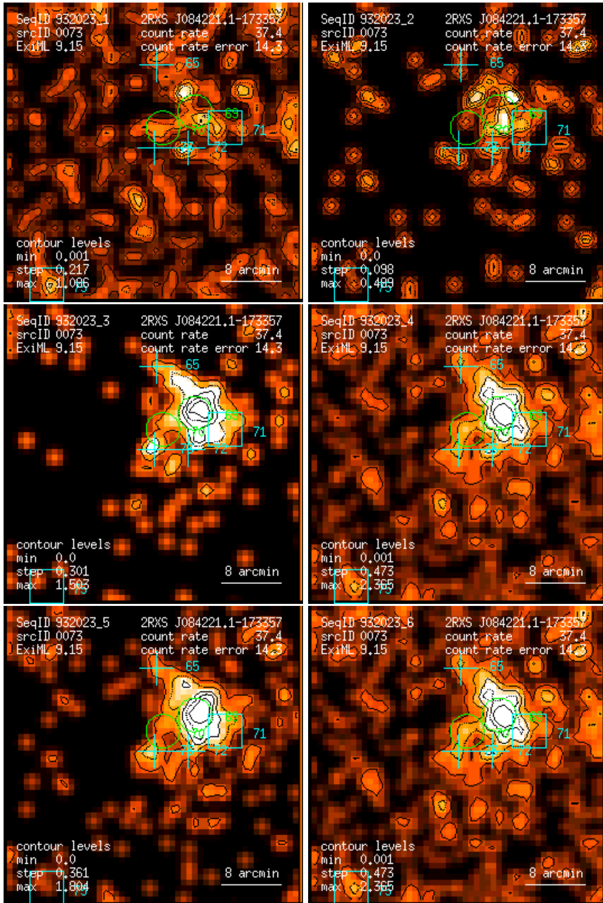
Figure 73: RASS 932023: detection 0073: band rate images, Gaussian filter: (1) PSPC channels 11 – 41, (2) 52 – 90, (3) 91 – 201, (4) 11 – 235, (5) 52 – 201, (6) 11 – 201. Broad band rates in counts/ks. Band rate contour levels in counts/ks/arcmin 2 .
