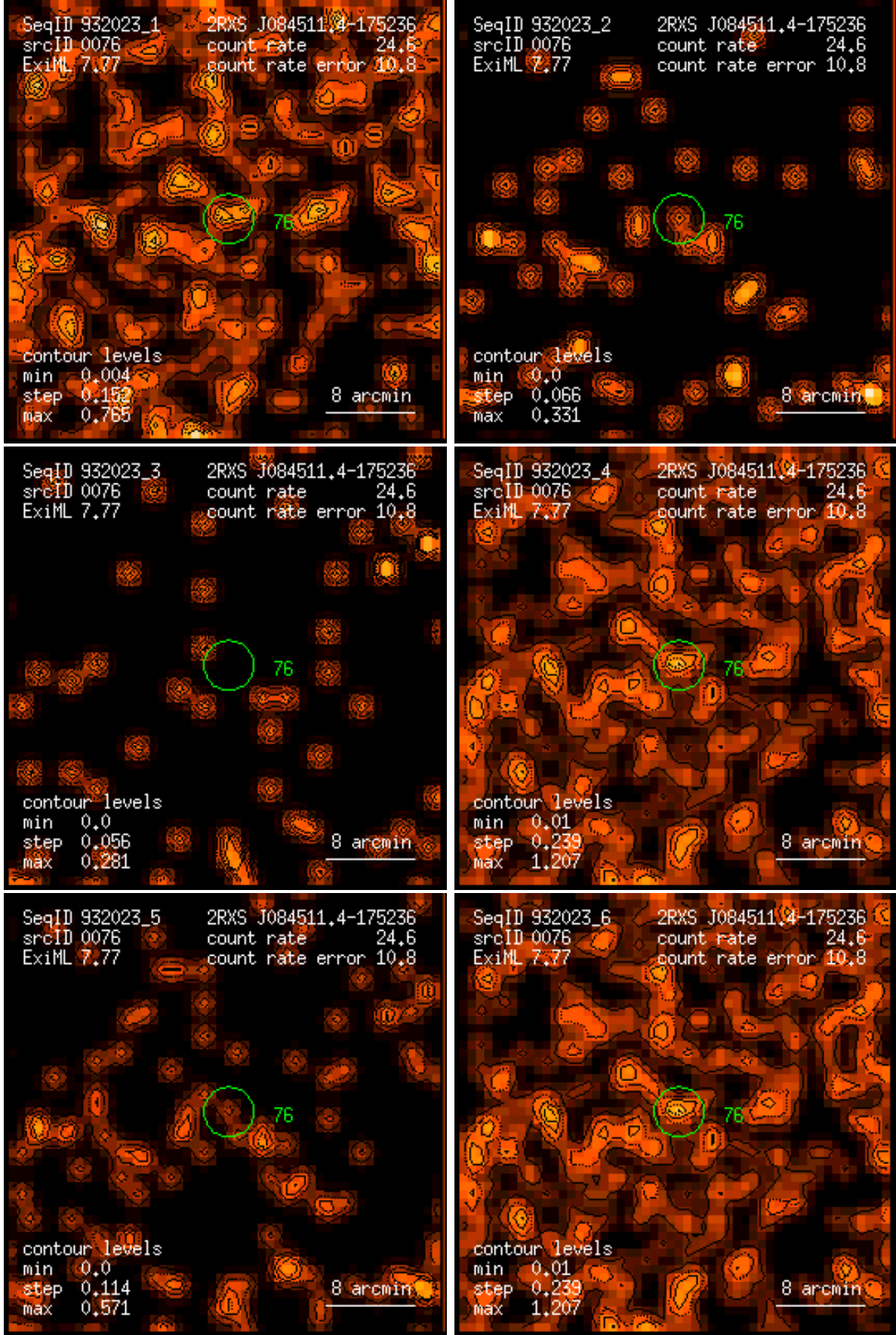
Figure 76: RASS 932023: detection 0076: band rate images, Gaussian filter: (1) PSPC channels 11 – 41, (2) 52 – 90, (3) 91 – 201, (4) 11 – 235, (5) 52 – 201, (6) 11 – 201. Broad band rates in counts/ks. Band rate contour levels in counts/ks/arcmin 2 .
