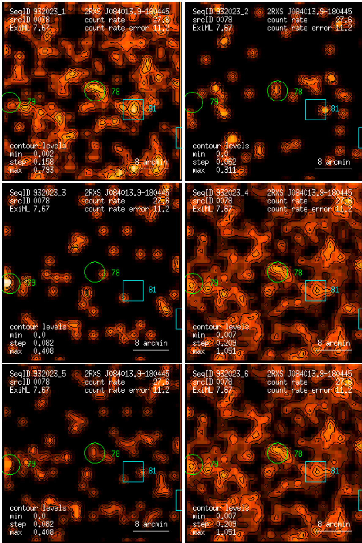
Figure 78: RASS 932023: detection 0078: band rate images, Gaussian filter: (1) PSPC channels 11 – 41, (2) 52 – 90, (3) 91 – 201, (4) 11 – 235, (5) 52 – 201, (6) 11 – 201. Broad band rates in counts/ks. Band rate contour levels in counts/ks/arcmin 2 .
