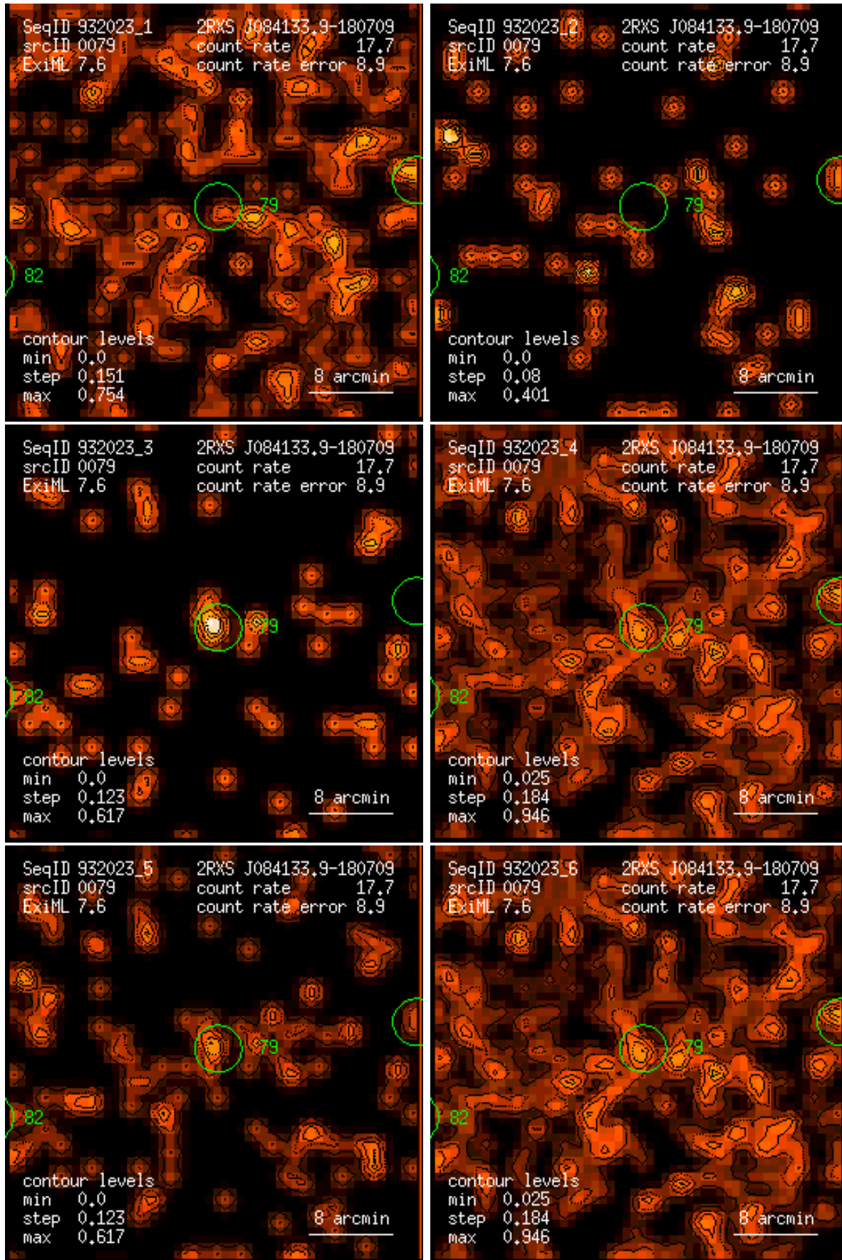
Figure 79: RASS 932023: detection 0079: band rate images, Gaussian filter: (1) PSPC channels 11 – 41, (2) 52 – 90, (3) 91 – 201, (4) 11 – 235, (5) 52 – 201, (6) 11 – 201. Broad band rates in counts/ks. Band rate contour levels in counts/ks/arcmin 2 .
