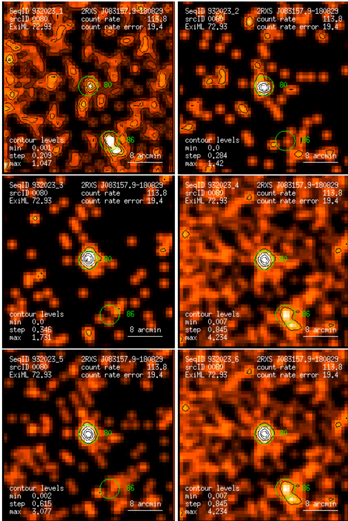
Figure 80: RASS 932023: detection 0080: band rate images, Gaussian filter: (1) PSPC channels 11 – 41, (2) 52 – 90, (3) 91 – 201, (4) 11 – 235, (5) 52 – 201, (6) 11 – 201. Broad band rates in counts/ks. Band rate contour levels in counts/ks/arcmin 2 .
