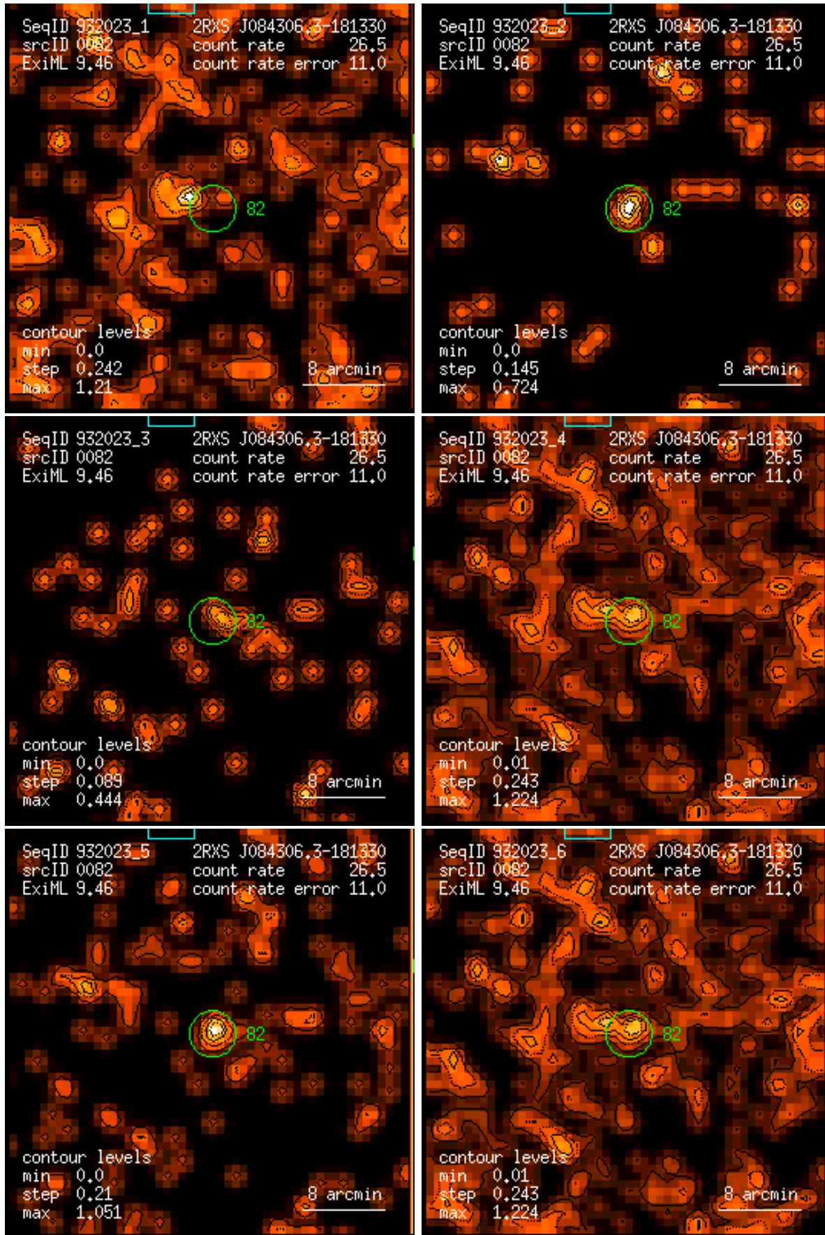
Figure 82: RASS 932023: detection 0082: band rate images, Gaussian filter: (1) PSPC channels 11 – 41, (2) 52 – 90, (3) 91 – 201, (4) 11 – 235, (5) 52 – 201, (6) 11 – 201. Broad band rates in counts/ks. Band rate contour levels in counts/ks/arcmin 2 .
