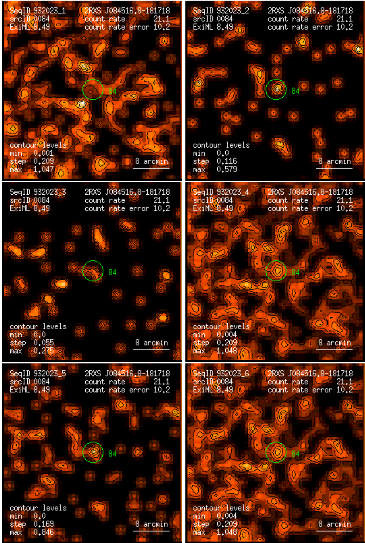
Figure 84: RASS 932023: detection 0084: band rate images, Gaussian filter: (1) PSPC channels 11 – 41, (2) 52 – 90, (3) 91 – 201, (4) 11 – 235, (5) 52 – 201, (6) 11 – 201. Broad band rates in counts/ks. Band rate contour levels in counts/ks/arcmin 2 .
