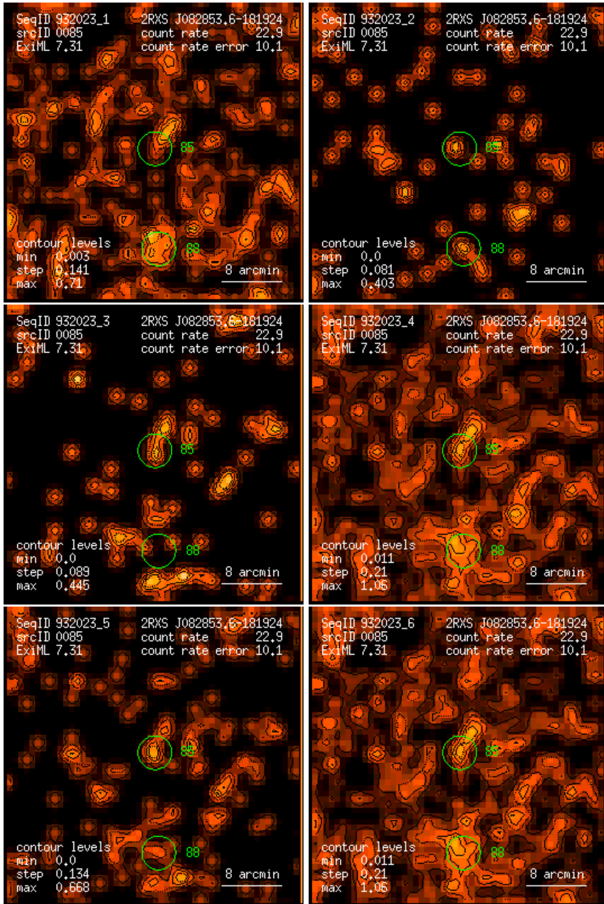
Figure 85: RASS 932023: detection 0085: band rate images, Gaussian filter: (1) PSPC channels 11 – 41, (2) 52 – 90, (3) 91 – 201, (4) 11 – 235, (5) 52 – 201, (6) 11 – 201. Broad band rates in counts/ks. Band rate contour levels in counts/ks/arcmin 2 .
