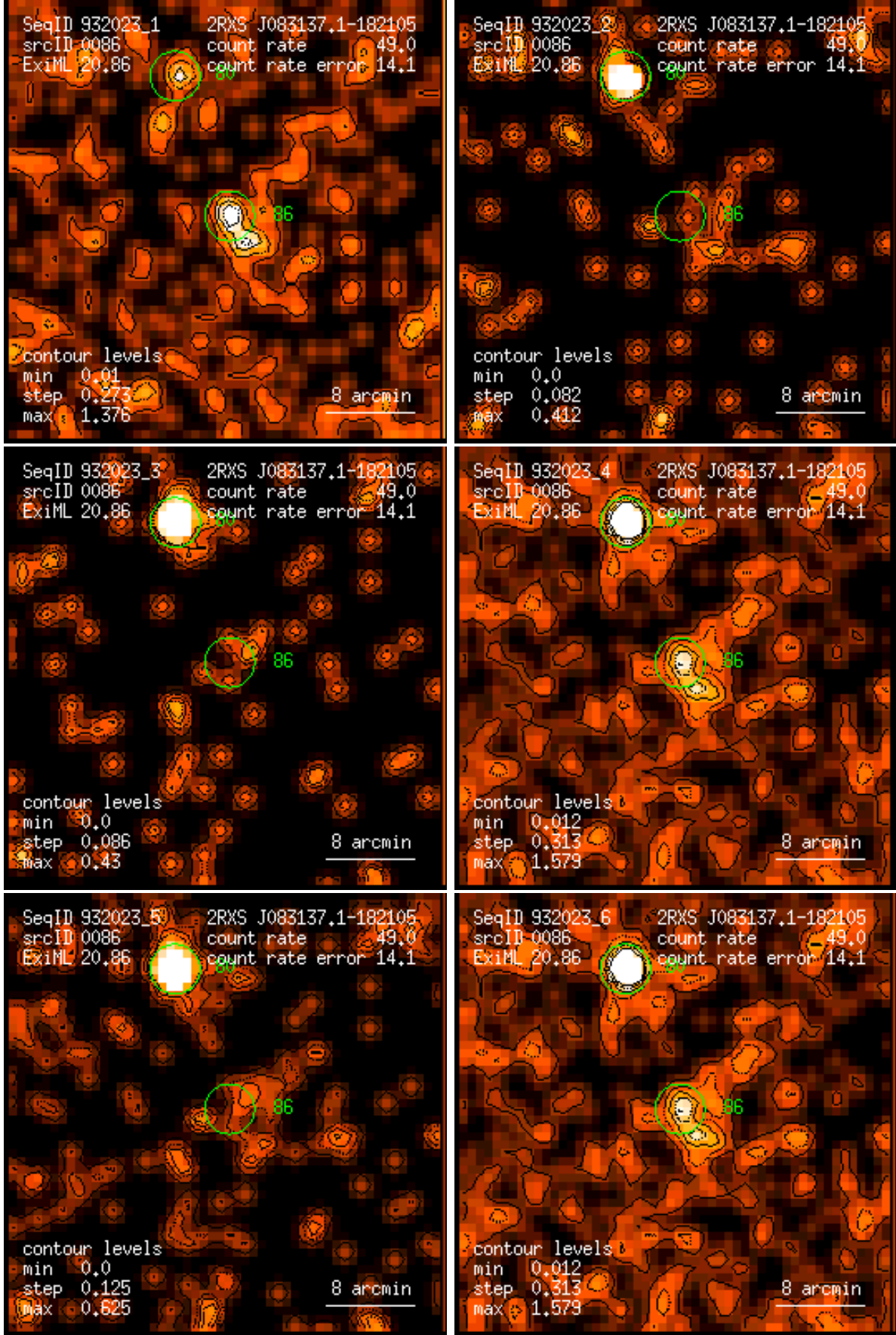
Figure 86: RASS 932023: detection 0086: band rate images, Gaussian filter: (1) PSPC channels 11 – 41, (2) 52 – 90, (3) 91 – 201, (4) 11 – 235, (5) 52 – 201, (6) 11 – 201. Broad band rates in counts/ks. Band rate contour levels in counts/ks/arcmin 2 .
