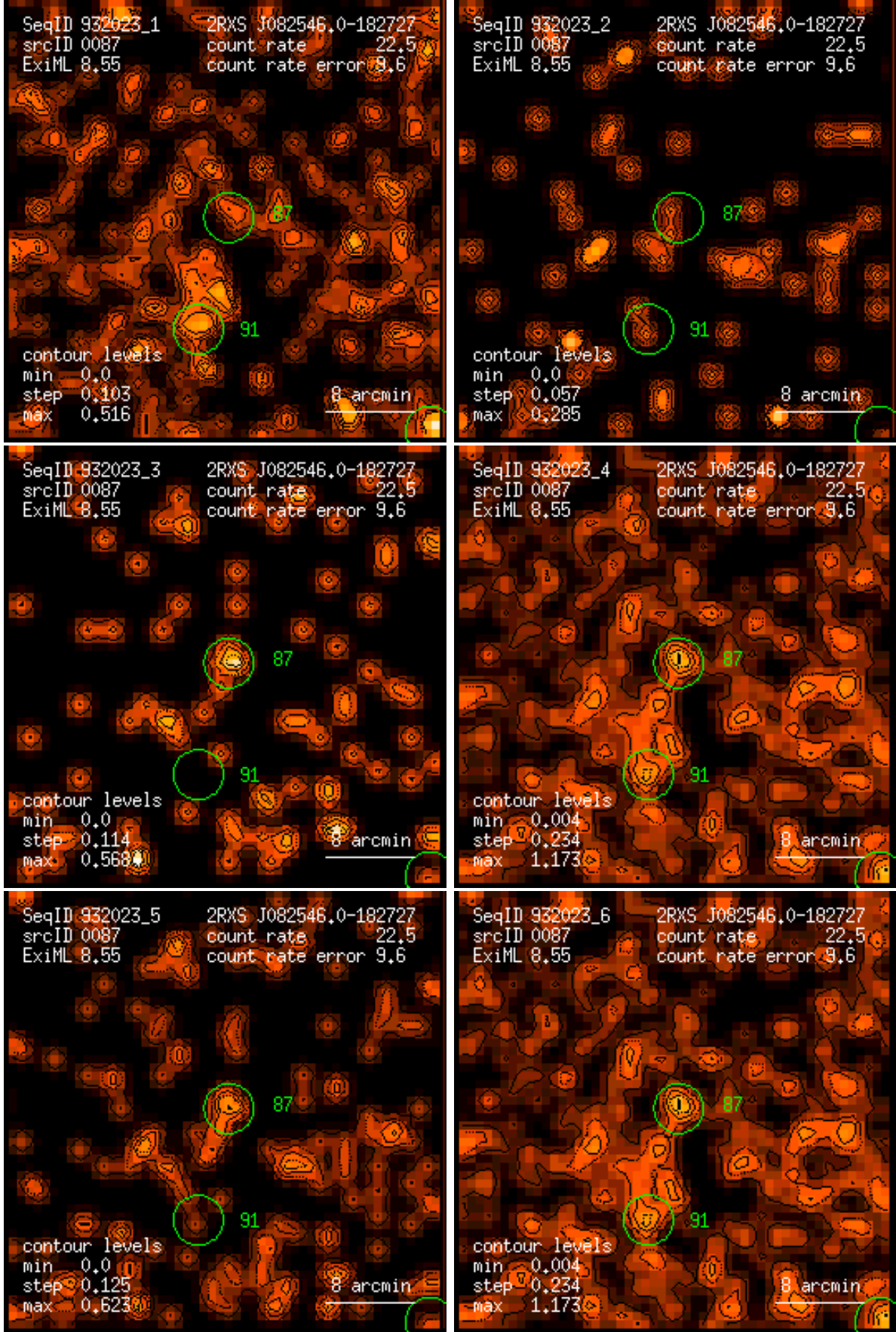
Figure 87: RASS 932023: detection 0087: band rate images, Gaussian filter: (1) PSPC channels 11 – 41, (2) 52 – 90, (3) 91 – 201, (4) 11 – 235, (5) 52 – 201, (6) 11 – 201. Broad band rates in counts/ks. Band rate contour levels in counts/ks/arcmin 2 .
