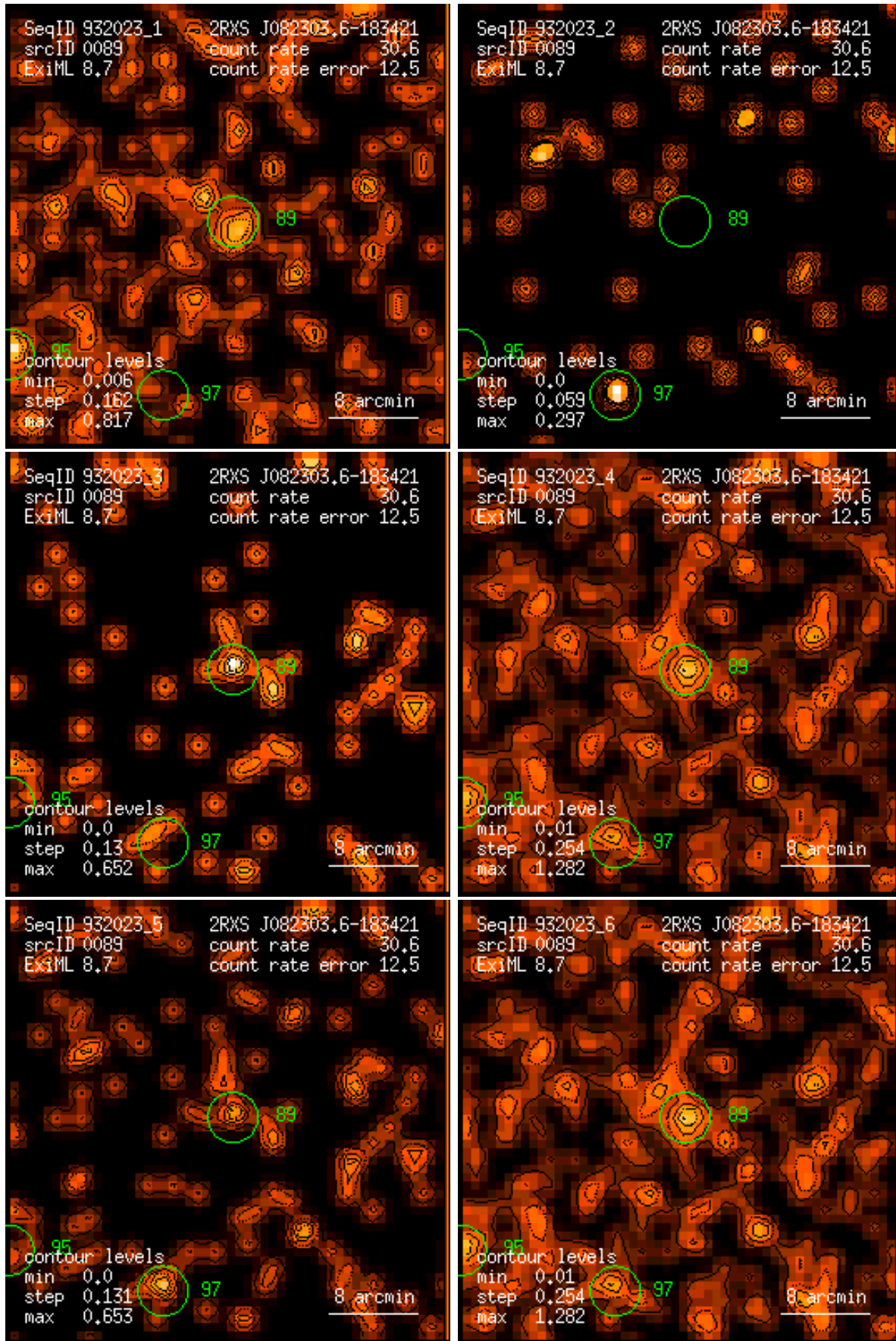
Figure 89: RASS 932023: detection 0089: band rate images, Gaussian filter: (1) PSPC channels 11 – 41, (2) 52 – 90, (3) 91 – 201, (4) 11 – 235, (5) 52 – 201, (6) 11 – 201. Broad band rates in counts/ks. Band rate contour levels in counts/ks/arcmin 2 .
