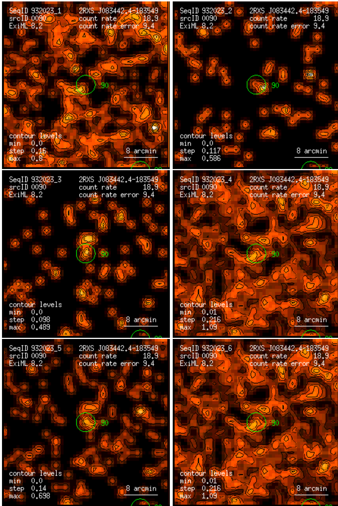
Figure 90: RASS 932023: detection 0090: band rate images, Gaussian filter: (1) PSPC channels 11 – 41, (2) 52 – 90, (3) 91 – 201, (4) 11 – 235, (5) 52 – 201, (6) 11 – 201. Broad band rates in counts/ks. Band rate contour levels in counts/ks/arcmin 2 .
