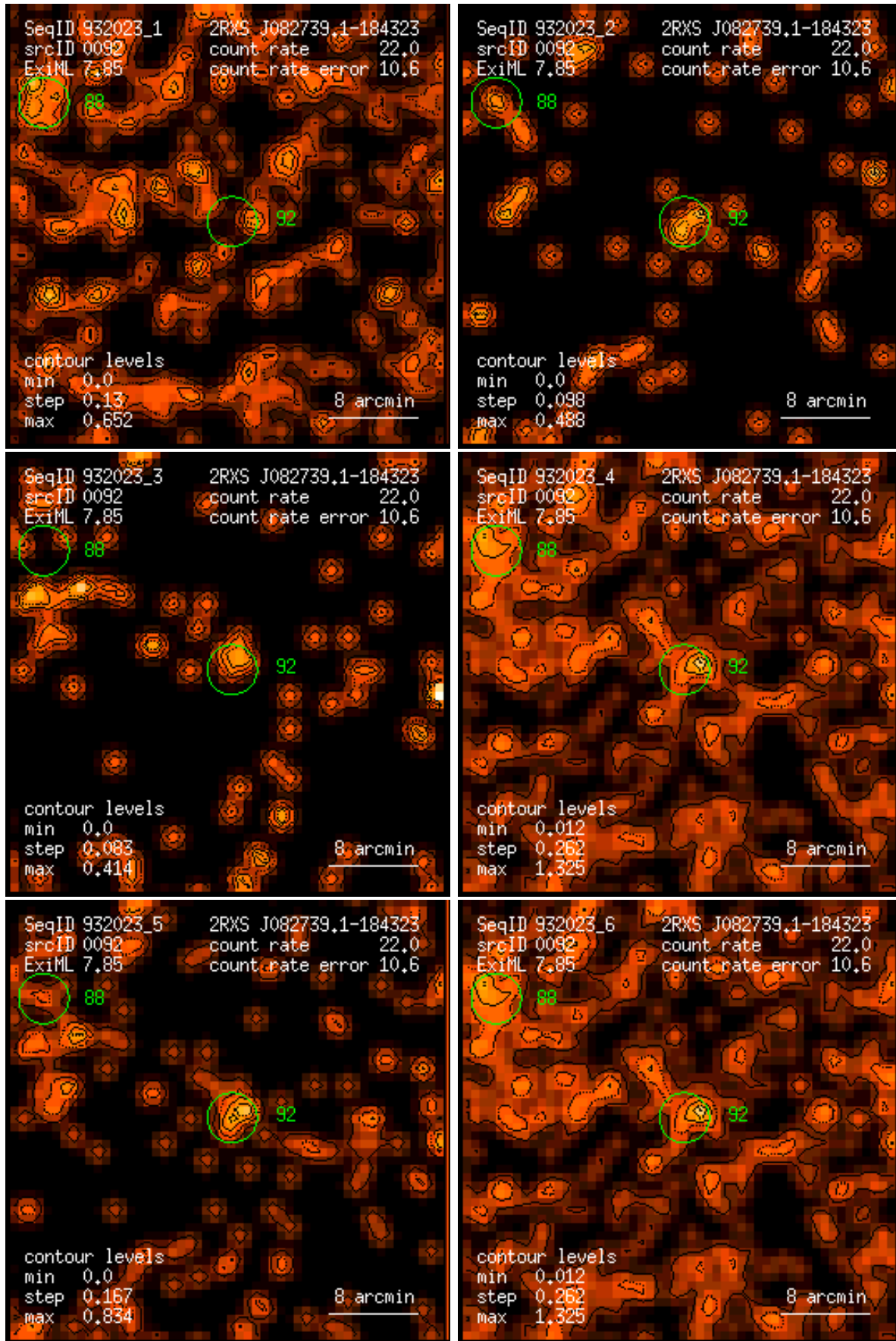
Figure 92: RASS 932023: detection 0092: band rate images, Gaussian filter: (1) PSPC channels 11 – 41, (2) 52 – 90, (3) 91 – 201, (4) 11 – 235, (5) 52 – 201, (6) 11 – 201. Broad band rates in counts/ks. Band rate contour levels in counts/ks/arcmin 2 .
