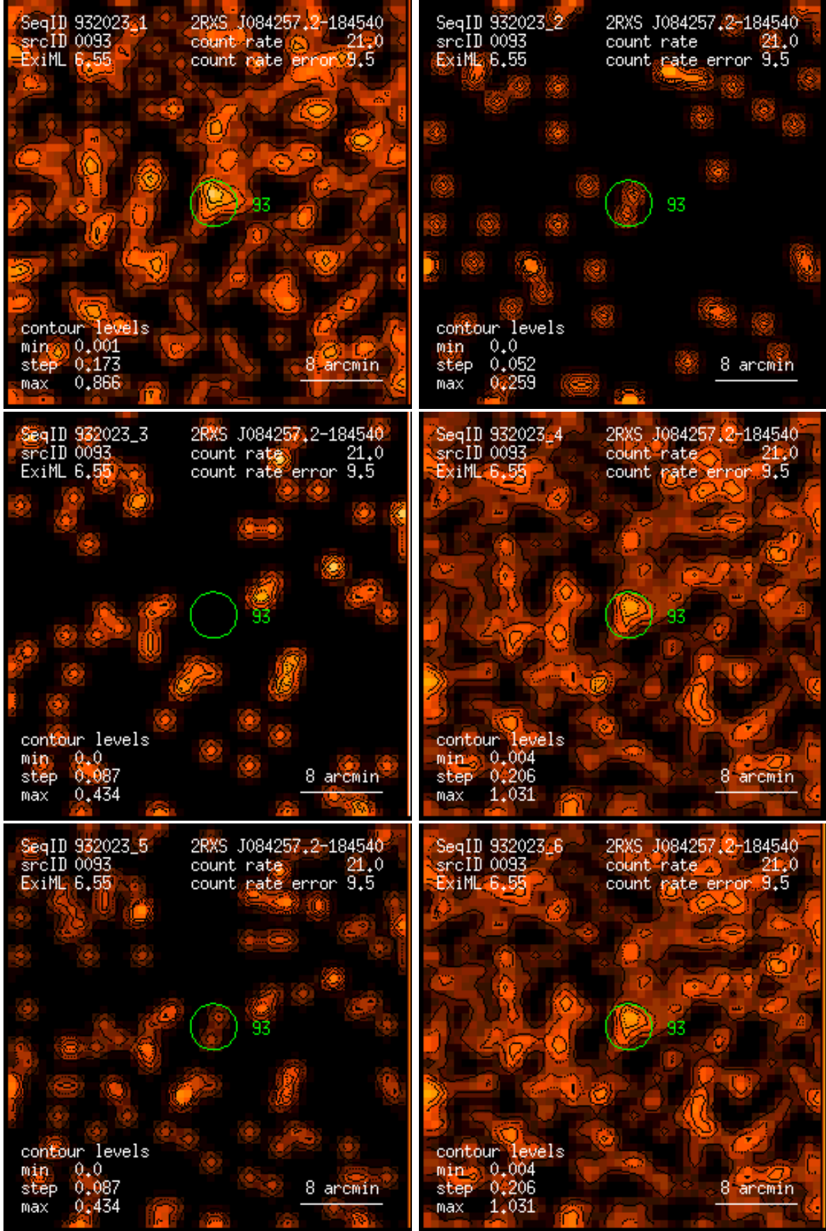
Figure 93: RASS 932023: detection 0093: band rate images, Gaussian filter: (1) PSPC channels 11 – 41, (2) 52 – 90, (3) 91 – 201, (4) 11 – 235, (5) 52 – 201, (6) 11 – 201. Broad band rates in counts/ks. Band rate contour levels in counts/ks/arcmin 2 .
