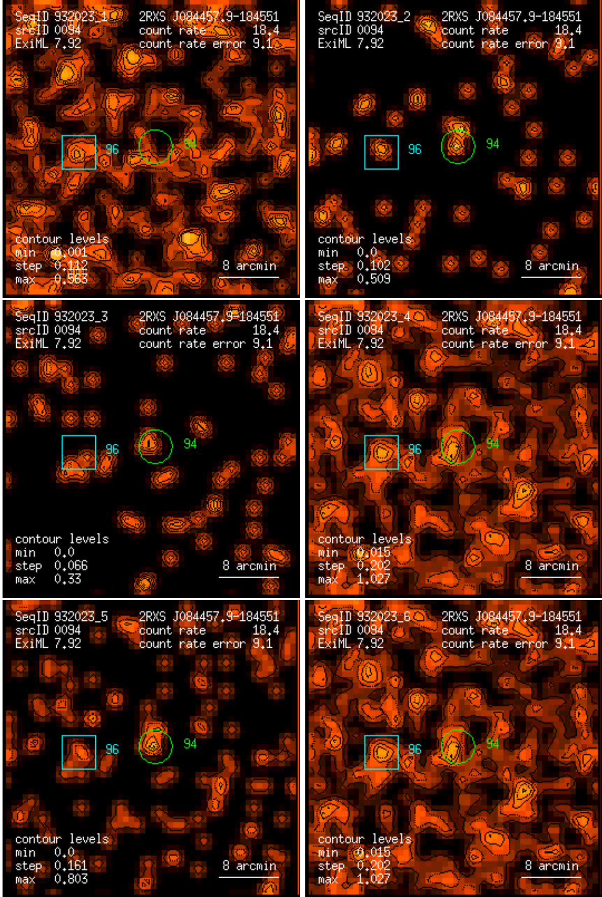
Figure 94: RASS 932023: detection 0094: band rate images, Gaussian filter: (1) PSPC channels 11 – 41, (2) 52 – 90, (3) 91 – 201, (4) 11 – 235, (5) 52 – 201, (6) 11 – 201. Broad band rates in counts/ks. Band rate contour levels in counts/ks/arcmin 2 .
