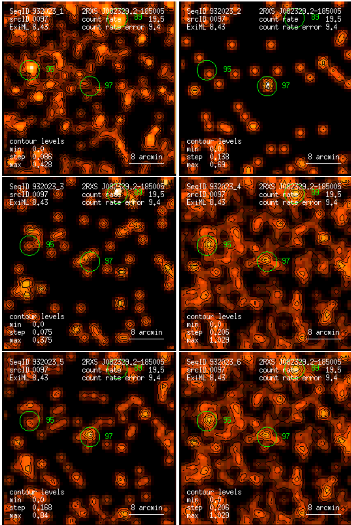
Figure 97: RASS 932023: detection 0097: band rate images, Gaussian filter: (1) PSPC channels 11 – 41, (2) 52 – 90, (3) 91 – 201, (4) 11 – 235, (5) 52 – 201, (6) 11 – 201. Broad band rates in counts/ks. Band rate contour levels in counts/ks/arcmin 2 .
