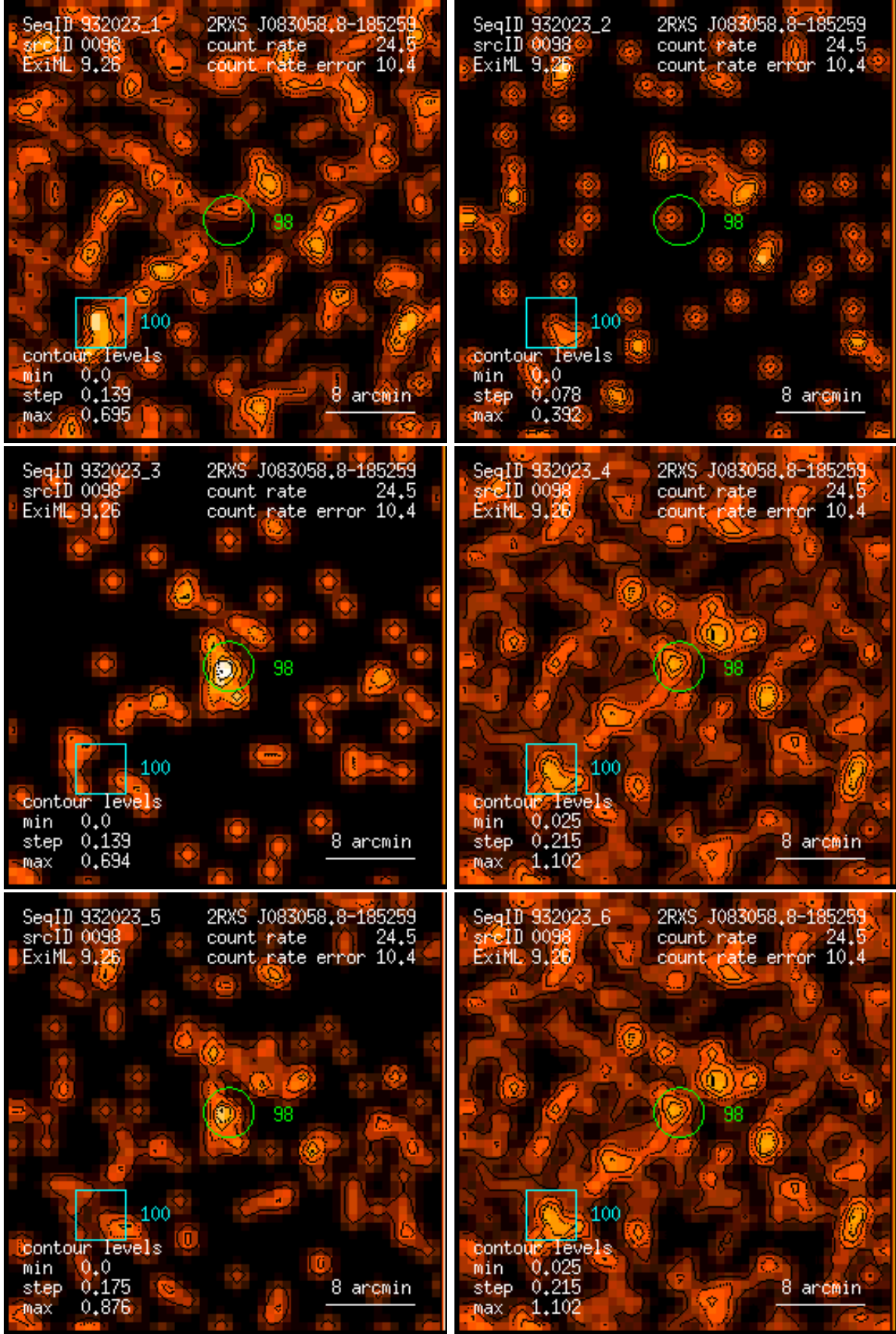
Figure 98: RASS 932023: detection 0098: band rate images, Gaussian filter: (1) PSPC channels 11 – 41, (2) 52 – 90, (3) 91 – 201, (4) 11 – 235, (5) 52 – 201, (6) 11 – 201. Broad band rates in counts/ks. Band rate contour levels in counts/ks/arcmin 2 .
