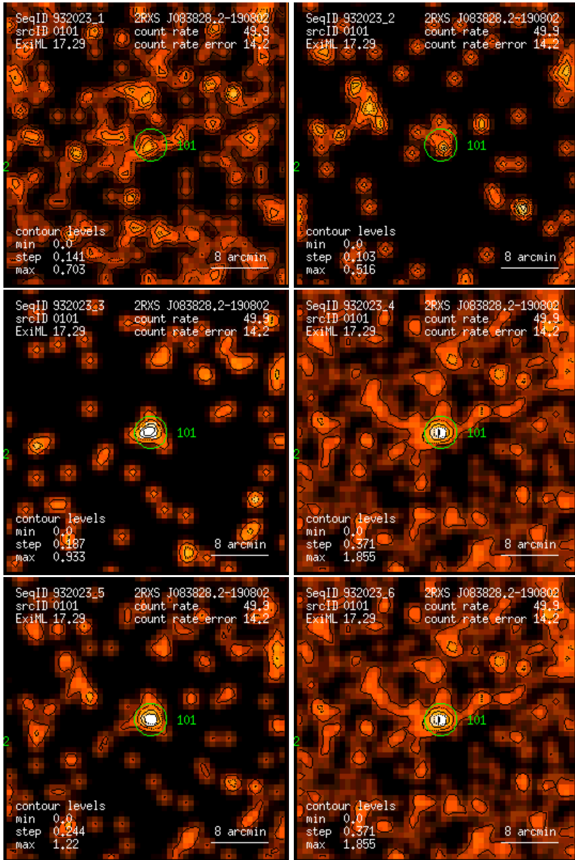
Figure 101: RASS 932023: detection 0101: band rate images, Gaussian filter: (1) PSPC channels 11 – 41, (2) 52 – 90, (3) 91 – 201, (4) 11 – 235, (5) 52 – 201, (6) 11 – 201. Broad band rates in counts/ks. Band rate contour levels in counts/ks/arcmin 2 .
