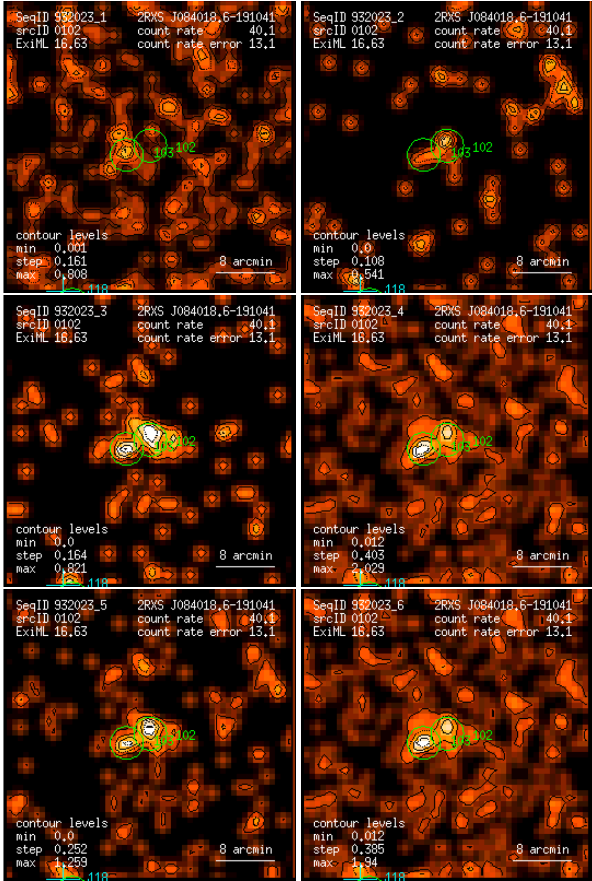
Figure 102: RASS 932023: detection 0102: band rate images, Gaussian filter: (1) PSPC channels 11 – 41, (2) 52 – 90, (3) 91 – 201, (4) 11 – 235, (5) 52 – 201, (6) 11 – 201. Broad band rates in counts/ks. Band rate contour levels in counts/ks/arcmin 2 .
