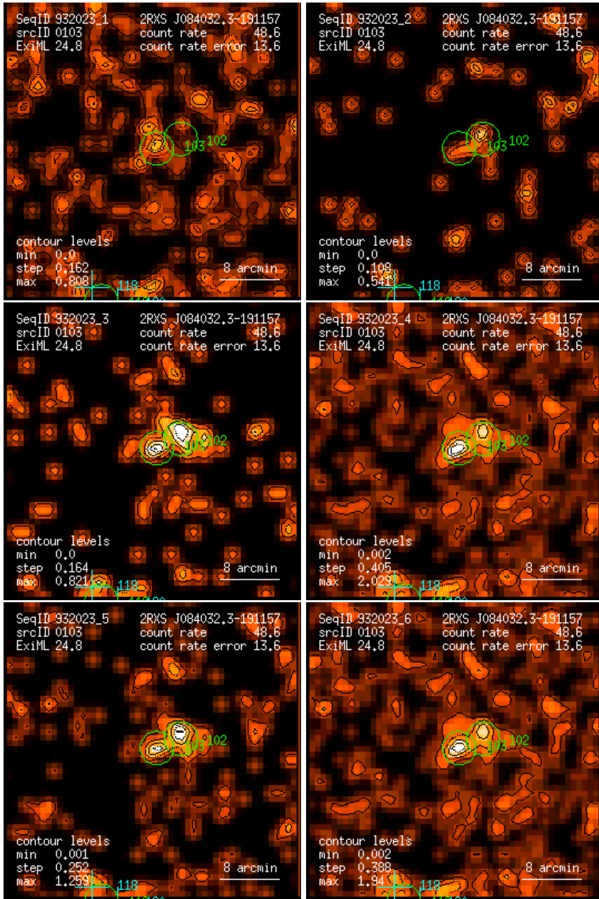
Figure 103: RASS 932023: detection 0103: band rate images, Gaussian filter: (1) PSPC channels 11 – 41, (2) 52 – 90, (3) 91 – 201, (4) 11 – 235, (5) 52 – 201, (6) 11 – 201. Broad band rates in counts/ks. Band rate contour levels in counts/ks/arcmin 2 .
