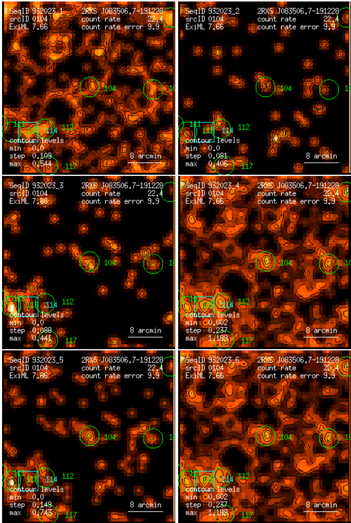
Figure 104: RASS 932023: detection 0104: band rate images, Gaussian filter: (1) PSPC channels 11 – 41, (2) 52 – 90, (3) 91 – 201, (4) 11 – 235, (5) 52 – 201, (6) 11 – 201. Broad band rates in counts/ks. Band rate contour levels in counts/ks/arcmin 2 .
