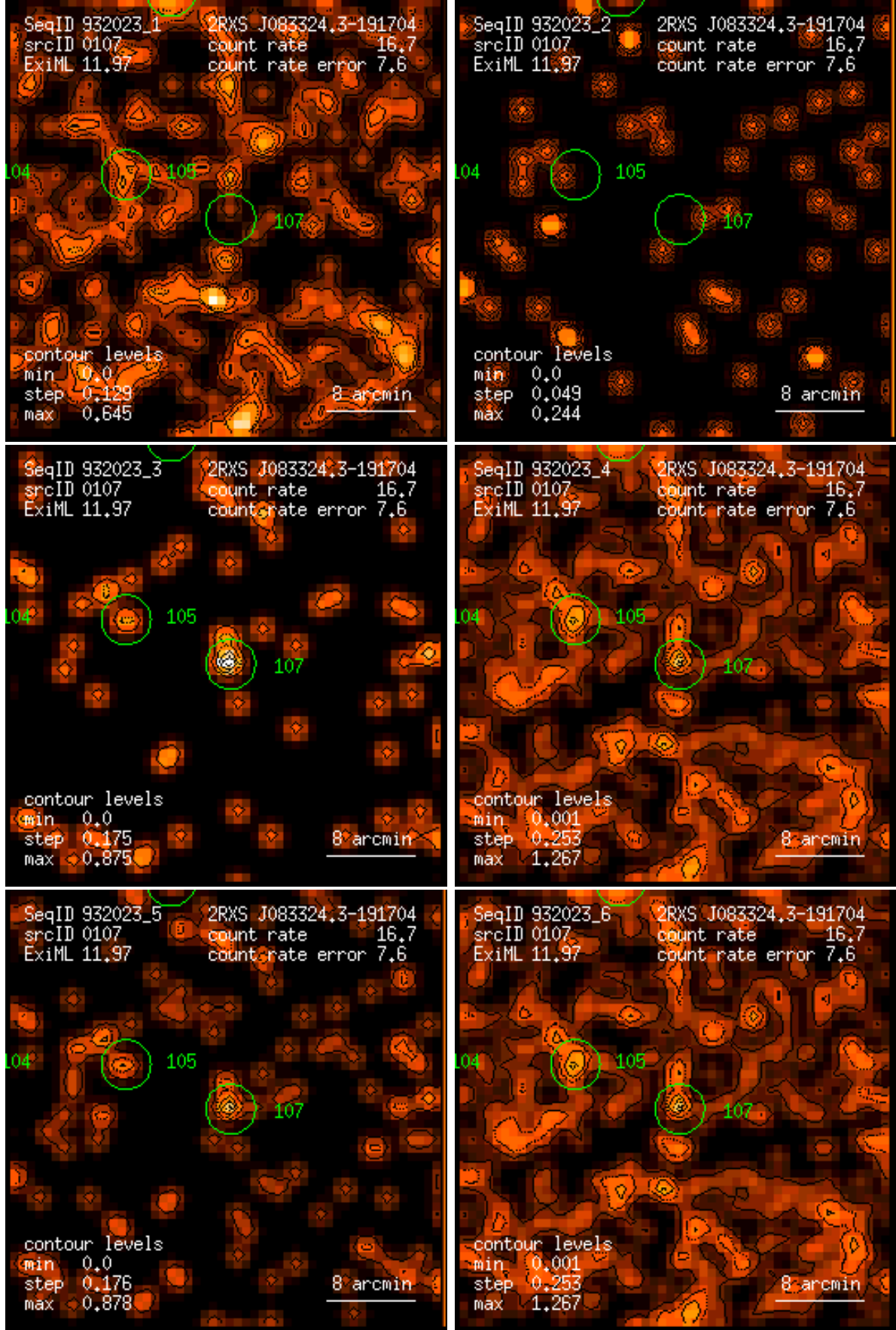
Figure 107: RASS 932023: detection 0107: band rate images, Gaussian filter: (1) PSPC channels 11 – 41, (2) 52 – 90, (3) 91 – 201, (4) 11 – 235, (5) 52 – 201, (6) 11 – 201. Broad band rates in counts/ks. Band rate contour levels in counts/ks/arcmin 2 .
