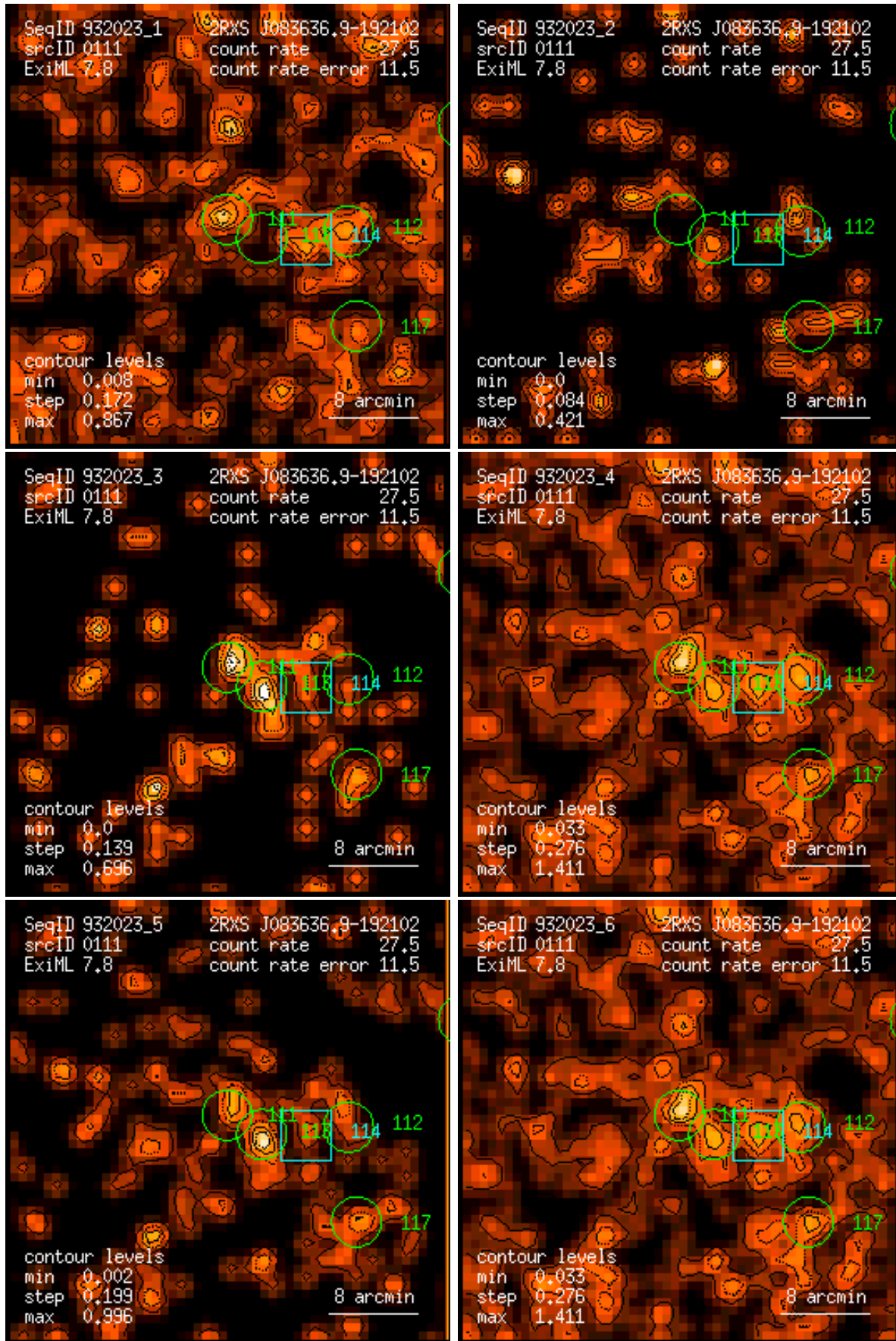
Figure 111: RASS 932023: detection 0111: band rate images, Gaussian filter: (1) PSPC channels 11 – 41, (2) 52 – 90, (3) 91 – 201, (4) 11 – 235, (5) 52 – 201, (6) 11 – 201. Broad band rates in counts/ks. Band rate contour levels in counts/ks/arcmin 2 .
