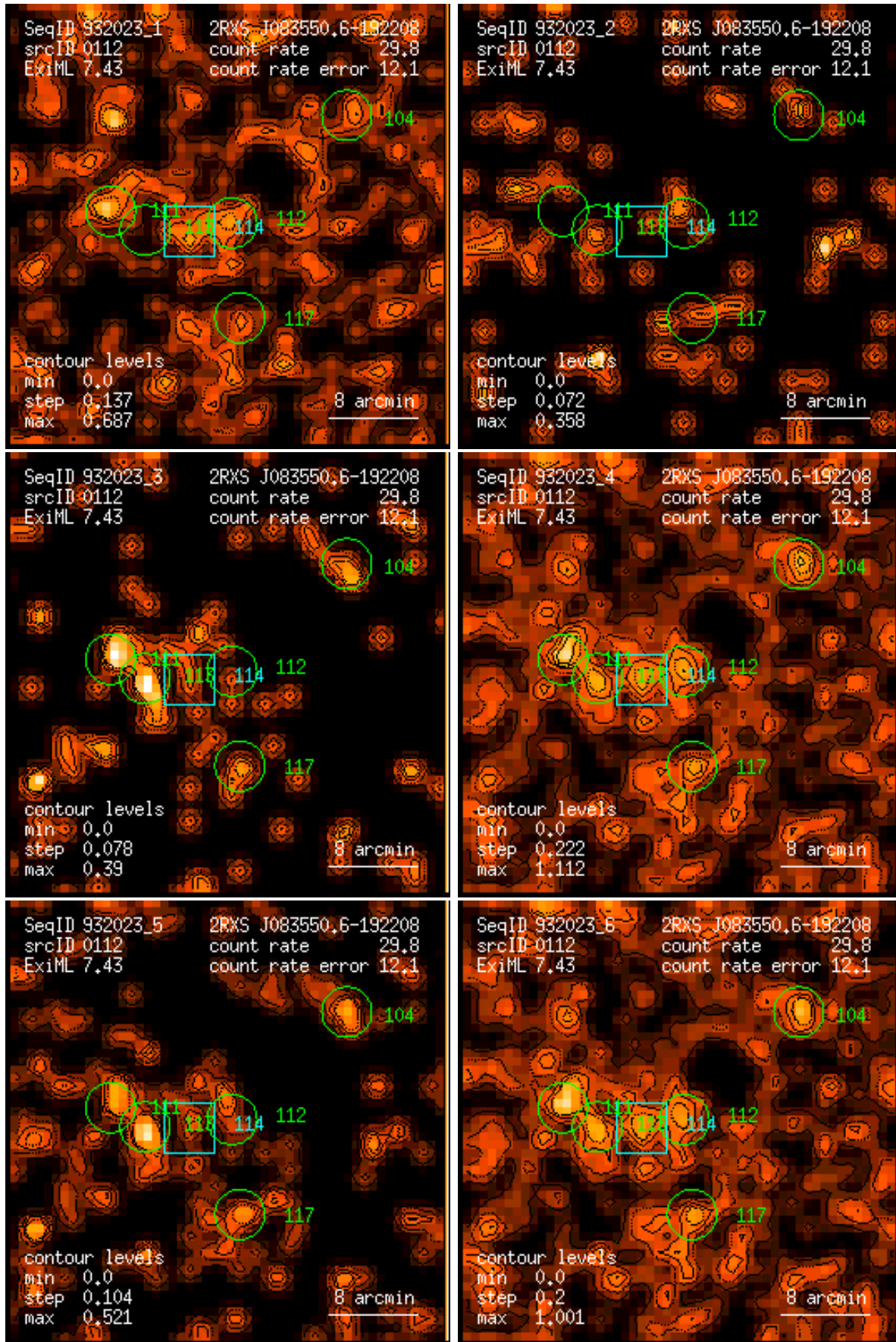
Figure 112: RASS 932023: detection 0112: band rate images, Gaussian filter: (1) PSPC channels 11 – 41, (2) 52 – 90, (3) 91 – 201, (4) 11 – 235, (5) 52 – 201, (6) 11 – 201. Broad band rates in counts/ks. Band rate contour levels in counts/ks/arcmin 2 .
