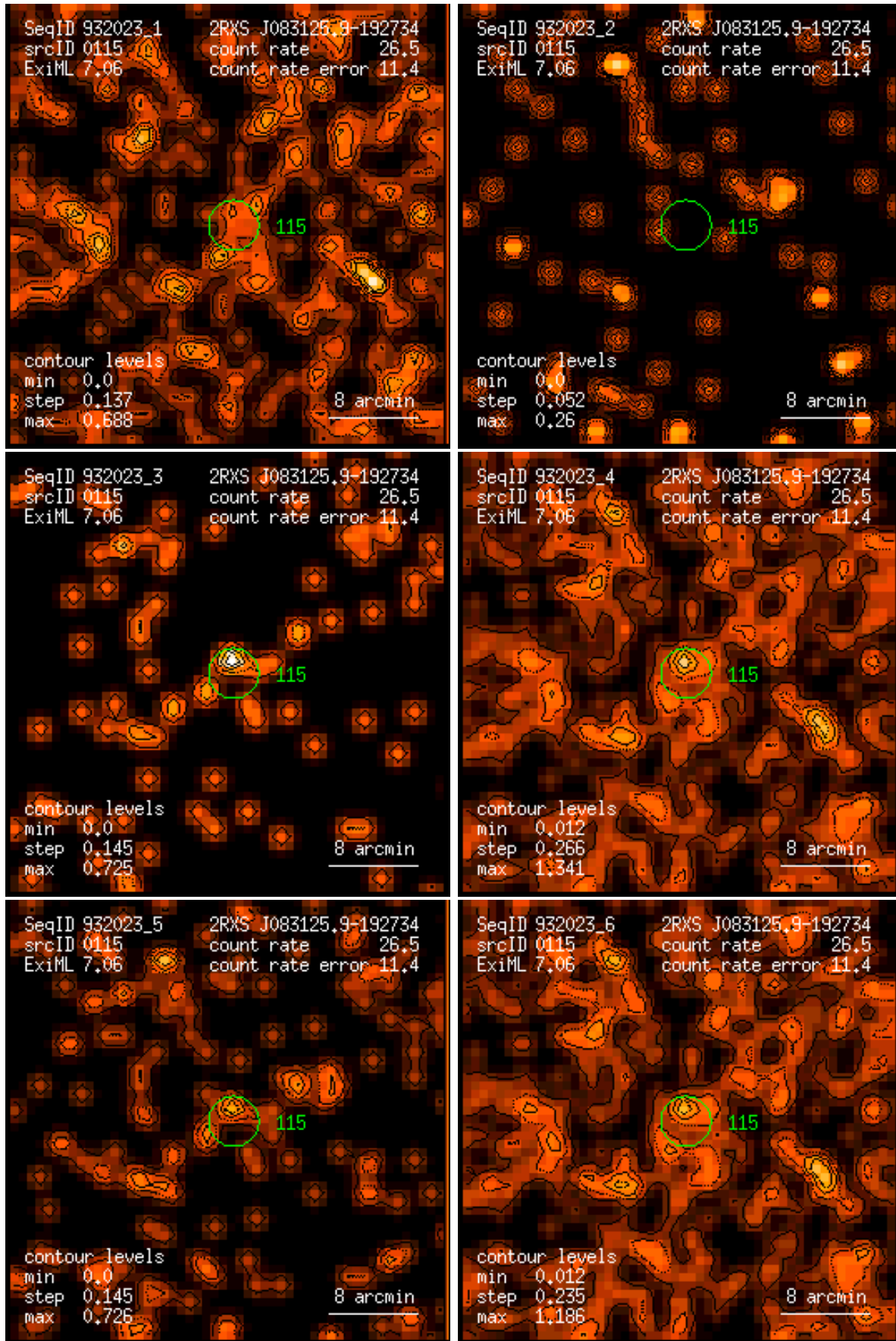
Figure 115: RASS 932023: detection 0115: band rate images, Gaussian filter: (1) PSPC channels 11 – 41, (2) 52 – 90, (3) 91 – 201, (4) 11 – 235, (5) 52 – 201, (6) 11 – 201. Broad band rates in counts/ks. Band rate contour levels in counts/ks/arcmin 2 .
