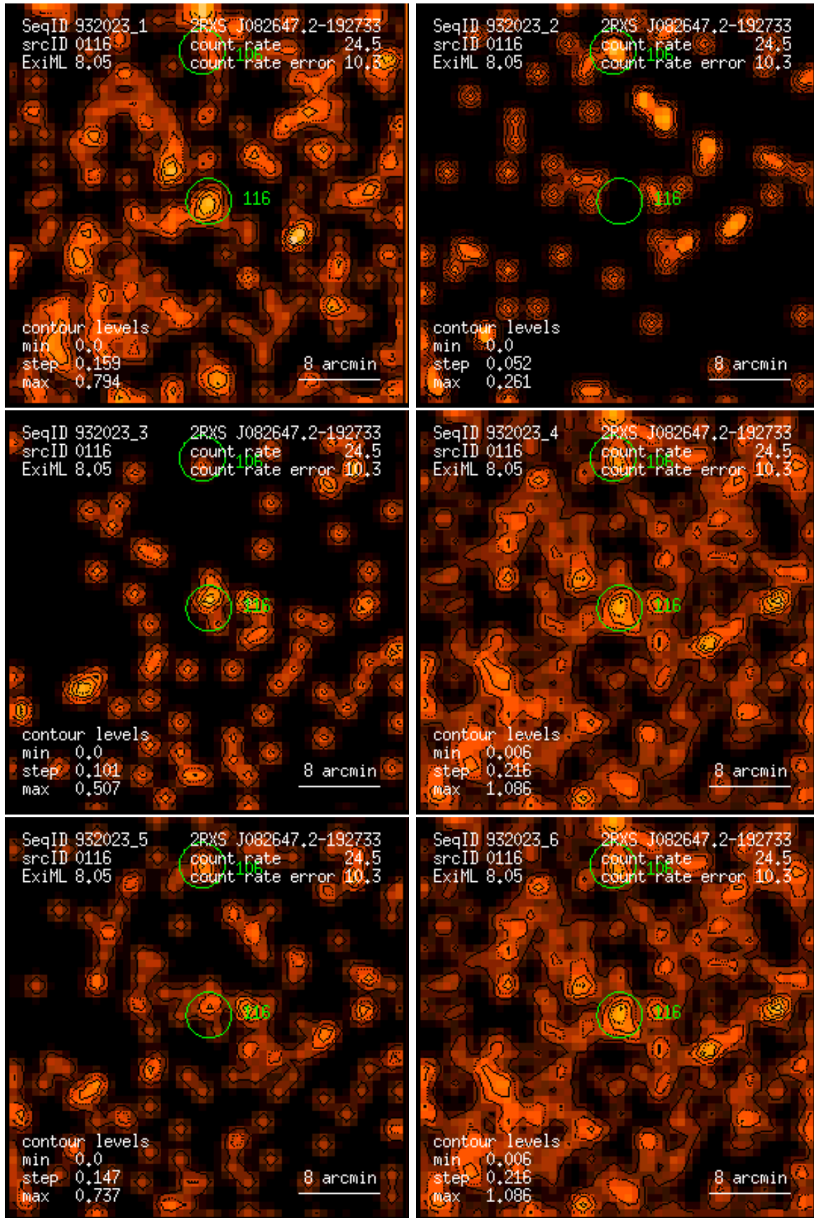
Figure 116: RASS 932023: detection 0116: band rate images, Gaussian filter: (1) PSPC channels 11 – 41, (2) 52 – 90, (3) 91 – 201, (4) 11 – 235, (5) 52 – 201, (6) 11 – 201. Broad band rates in counts/ks. Band rate contour levels in counts/ks/arcmin 2 .
