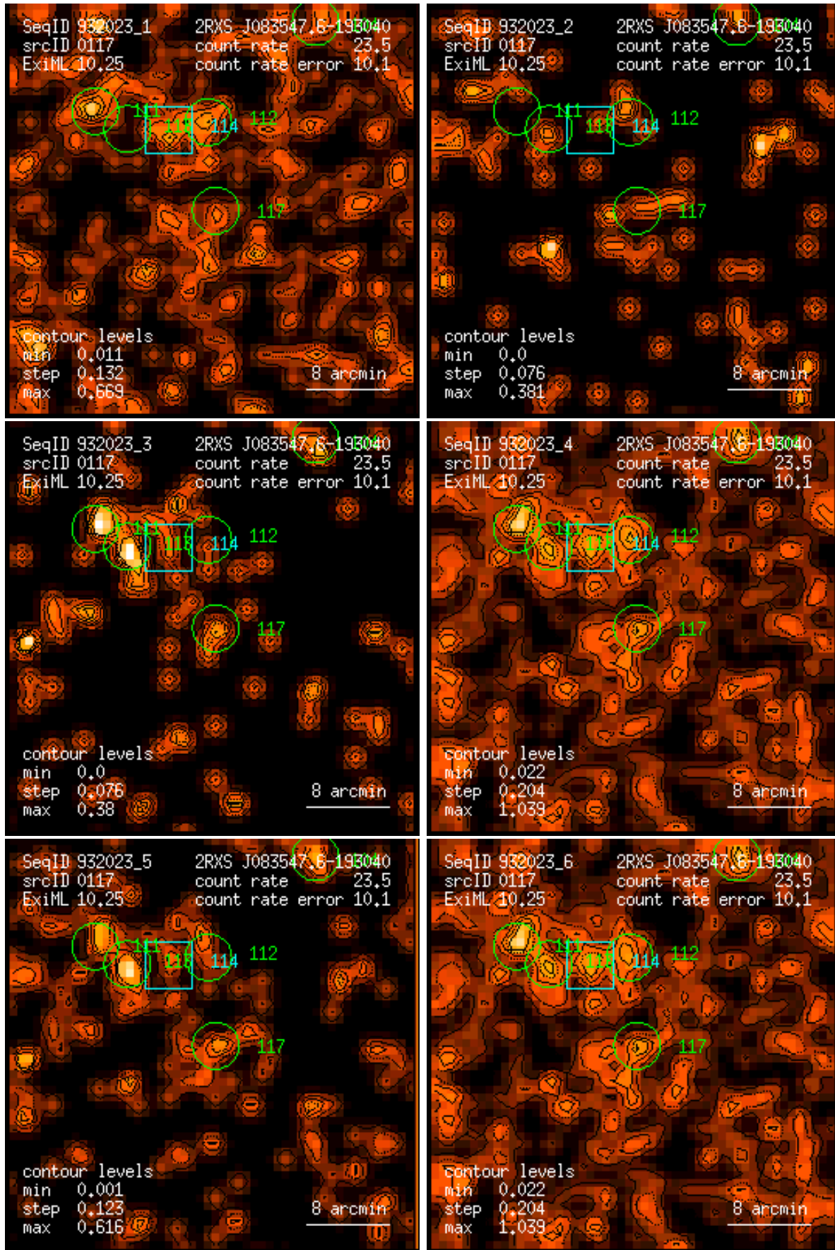
Figure 117: RASS 932023: detection 0117: band rate images, Gaussian filter: (1) PSPC channels 11 – 41, (2) 52 – 90, (3) 91 – 201, (4) 11 – 235, (5) 52 – 201, (6) 11 – 201. Broad band rates in counts/ks. Band rate contour levels in counts/ks/arcmin 2 .
