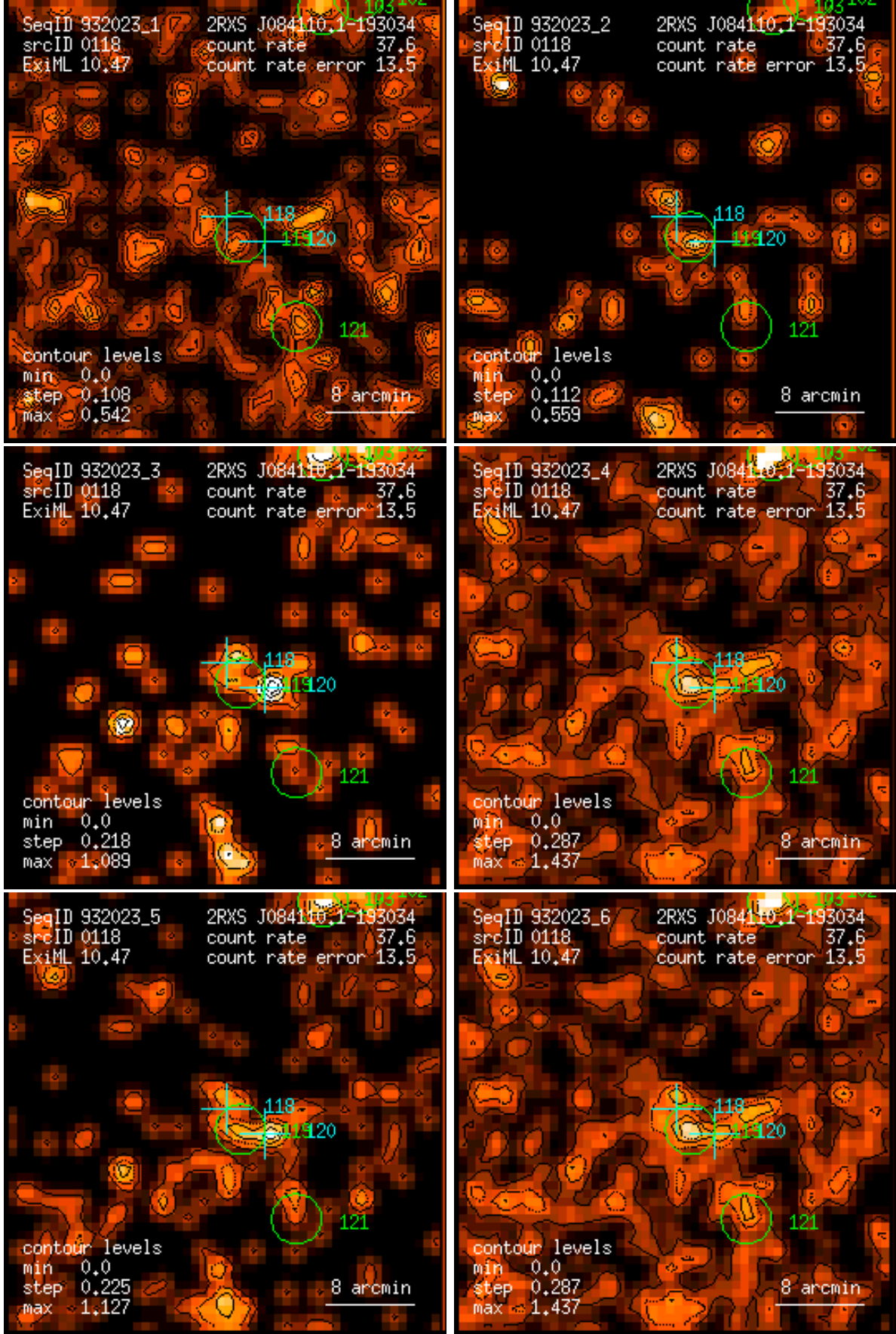
Figure 118: RASS 932023: detection 0118: band rate images, Gaussian filter: (1) PSPC channels 11 – 41, (2) 52 – 90, (3) 91 – 201, (4) 11 – 235, (5) 52 – 201, (6) 11 – 201. Broad band rates in counts/ks. Band rate contour levels in counts/ks/arcmin 2 .
