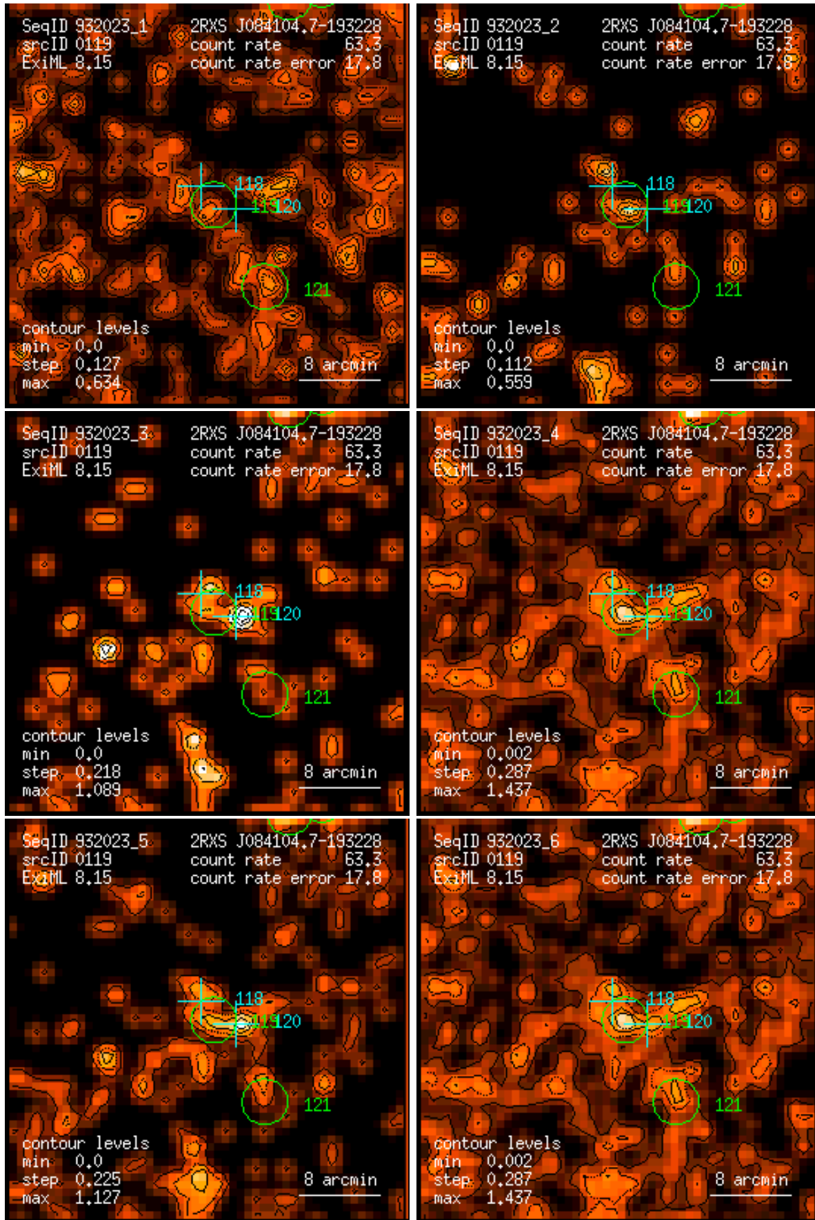
Figure 119: RASS 932023: detection 0119: band rate images, Gaussian filter: (1) PSPC channels 11 – 41, (2) 52 – 90, (3) 91 – 201, (4) 11 – 235, (5) 52 – 201, (6) 11 – 201. Broad band rates in counts/ks. Band rate contour levels in counts/ks/arcmin 2 .
