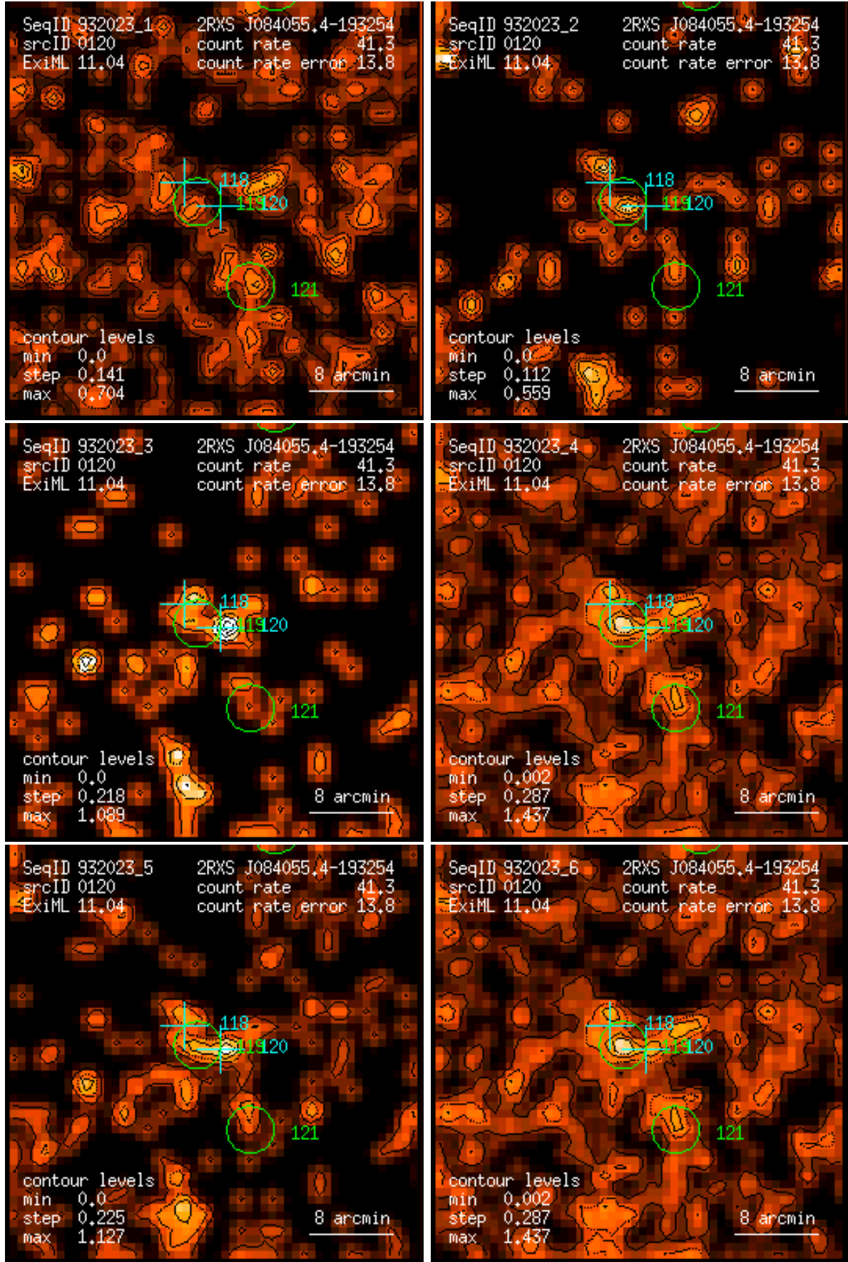
Figure 120: RASS 932023: detection 0120: band rate images, Gaussian filter: (1) PSPC channels 11 – 41, (2) 52 – 90, (3) 91 – 201, (4) 11 – 235, (5) 52 – 201, (6) 11 – 201. Broad band rates in counts/ks. Band rate contour levels in counts/ks/arcmin 2 .
