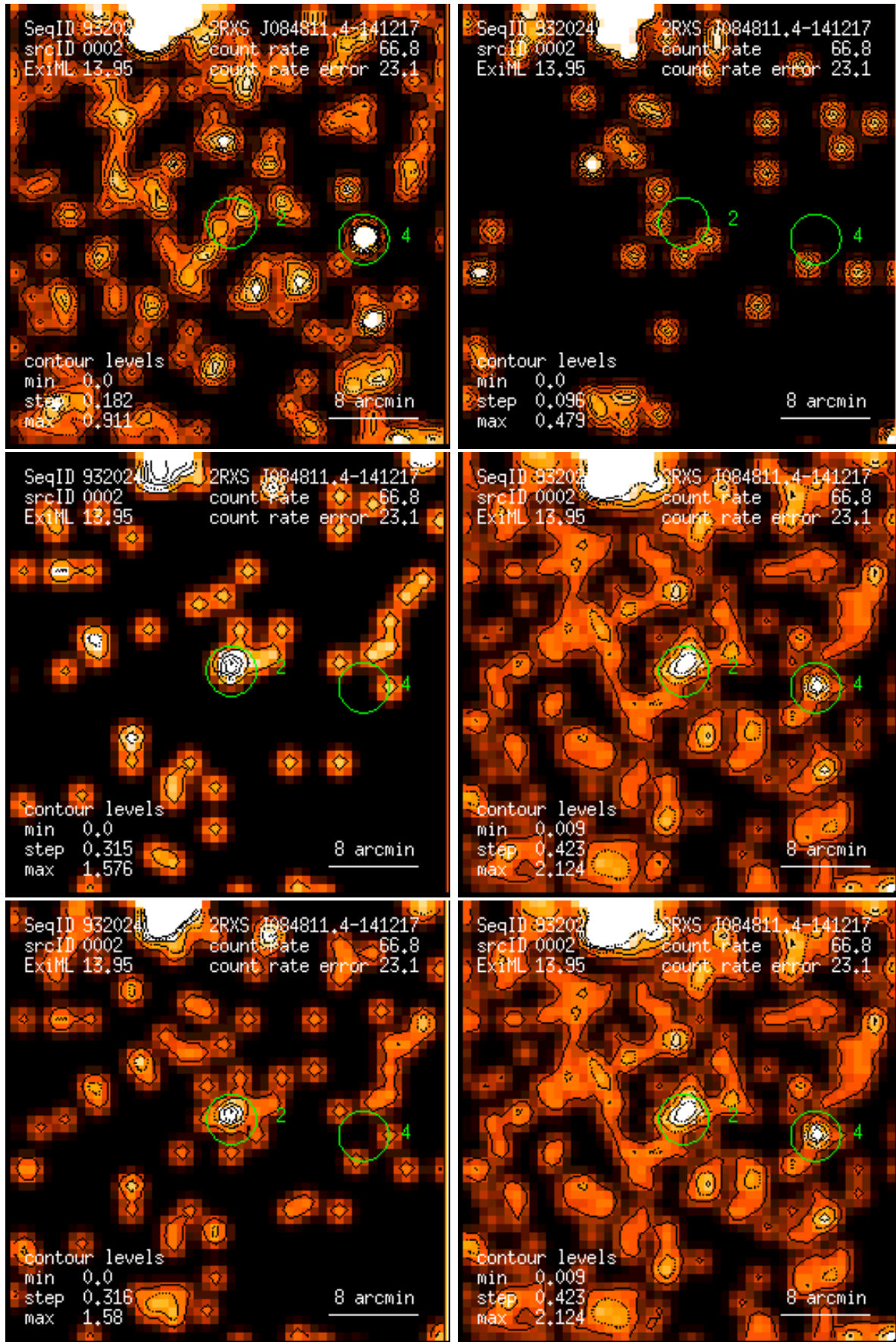
Figure 2: RASS 932024: detection 0002: band rate images, Gaussian filter: (1) PSPC channels 11 – 41, (2) 52 – 90, (3) 91 – 201, (4) 11 – 235, (5) 52 – 201, (6) 11 – 201. Broad band rates in counts/ks. Band rate contour levels in counts/ks/arcmin 2 .
