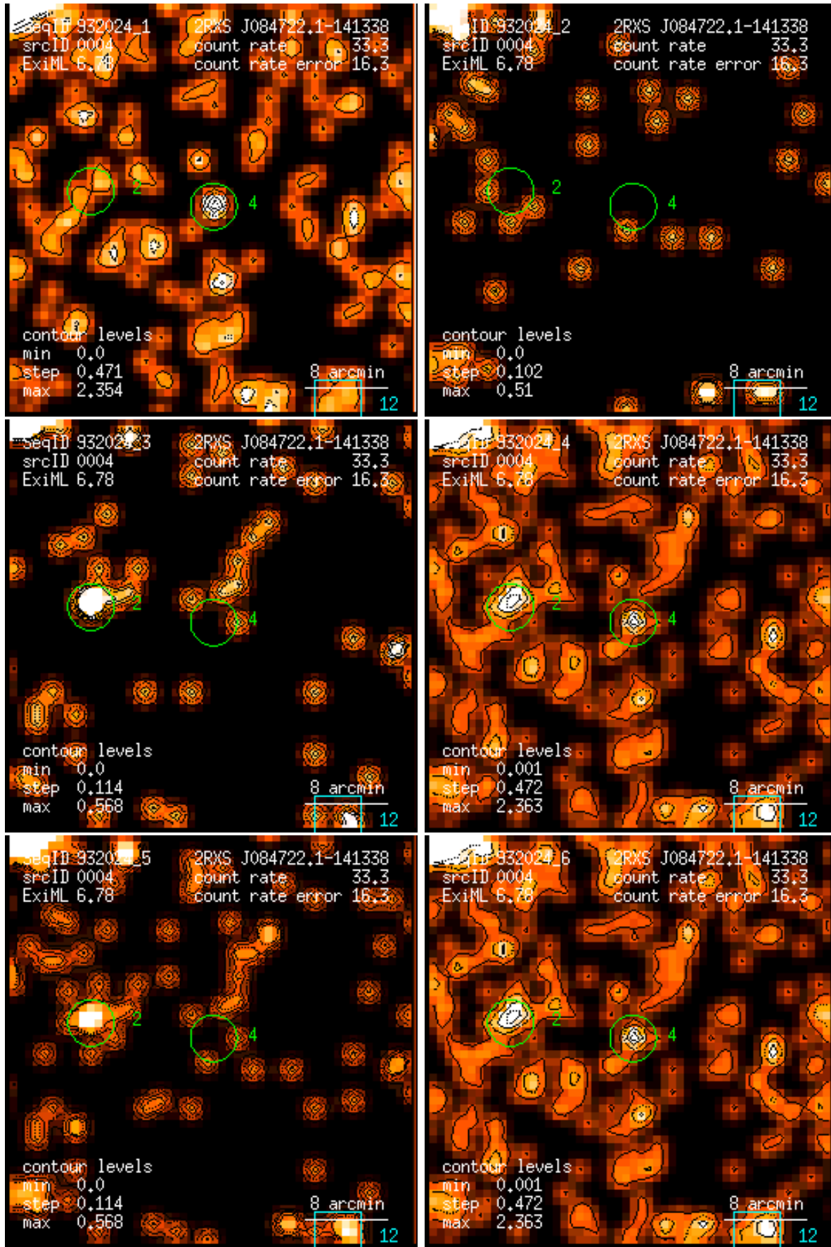
Figure 4: RASS 932024: detection 0004: band rate images, Gaussian filter: (1) PSPC channels 11 – 41, (2) 52 – 90, (3) 91 – 201, (4) 11 – 235, (5) 52 – 201, (6) 11 – 201. Broad band rates in counts/ks. Band rate contour levels in counts/ks/arcmin 2 .
