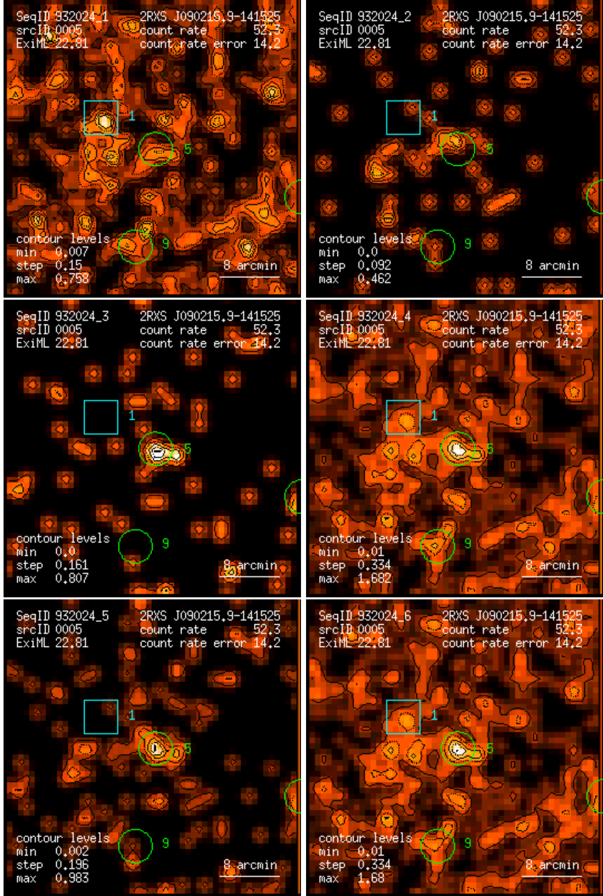
Figure 5: RASS 932024: detection 0005: band rate images, Gaussian filter: (1) PSPC channels 11 – 41, (2) 52 – 90, (3) 91 – 201, (4) 11 – 235, (5) 52 – 201, (6) 11 – 201. Broad band rates in counts/ks. Band rate contour levels in counts/ks/arcmin 2 .
