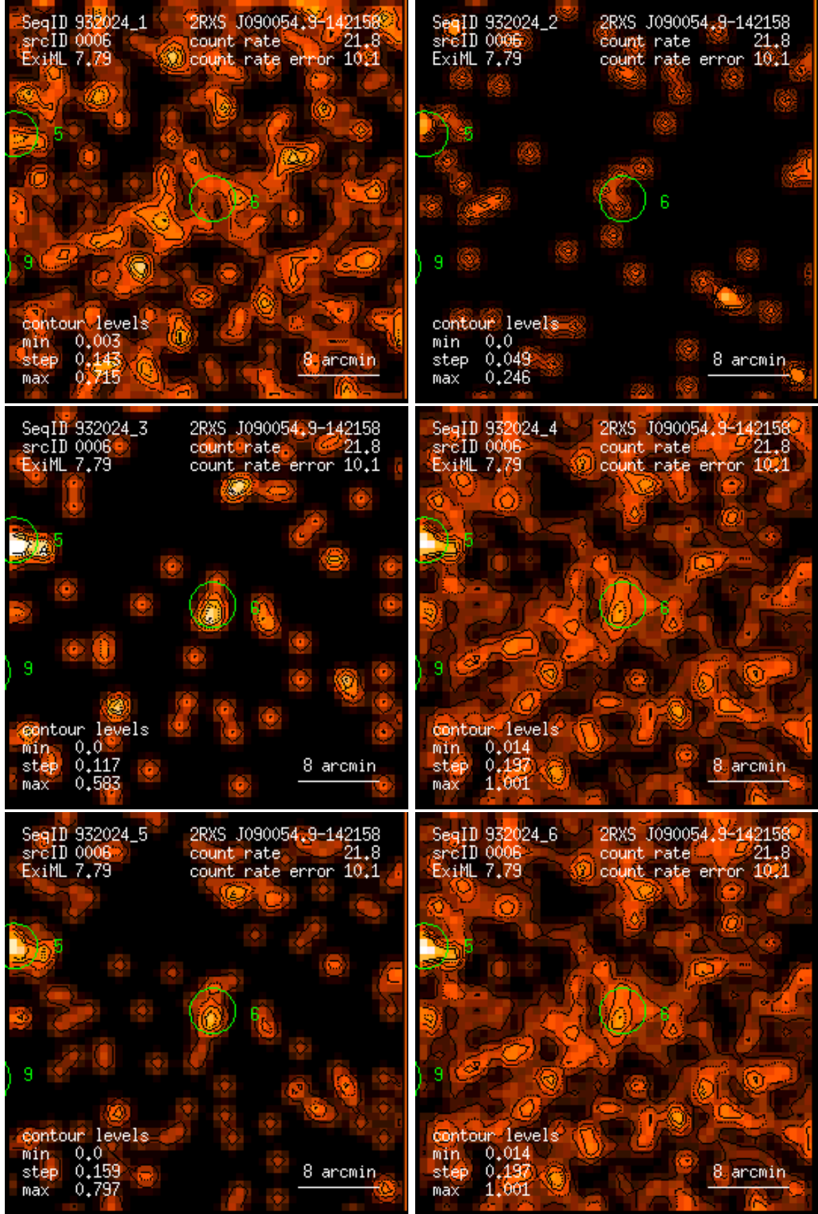
Figure 6: RASS 932024: detection 0006: band rate images, Gaussian filter: (1) PSPC channels 11 – 41, (2) 52 – 90, (3) 91 – 201, (4) 11 – 235, (5) 52 – 201, (6) 11 – 201. Broad band rates in counts/ks. Band rate contour levels in counts/ks/arcmin 2 .
